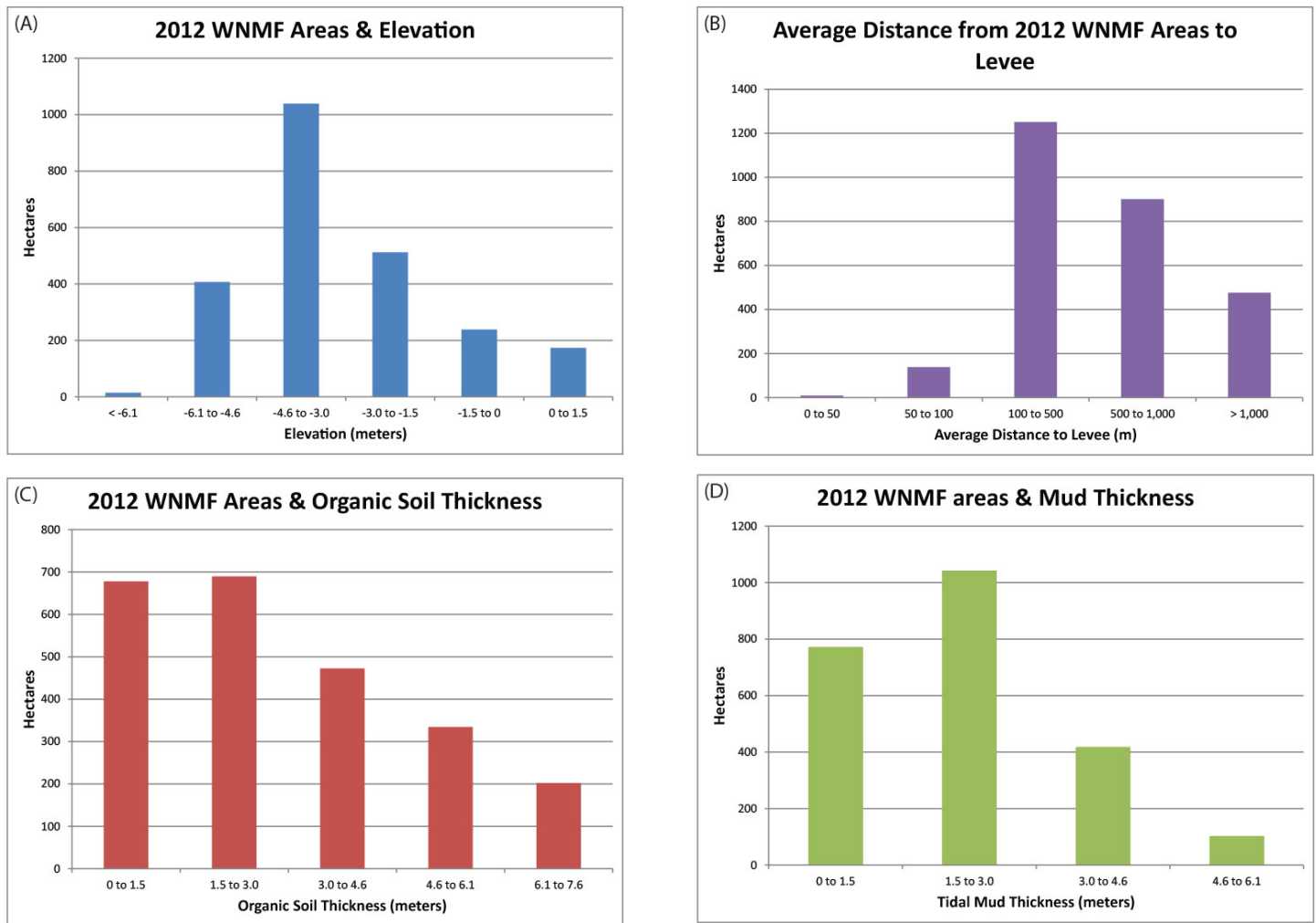
Figure 10 Histograms for 2012 WNMF areas: (A) elevation, (B) average distance from levee, (C) organic soil thickness, and (D) tidal mud thickness
