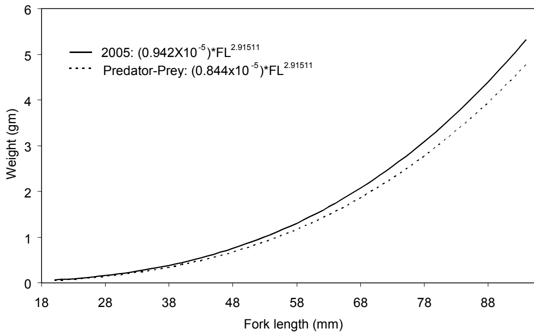
Figure 5. Inland silverside length-weight relationships from 2005 sampling and the Predator-Prey Study. Data points have been omitted for clarity.
