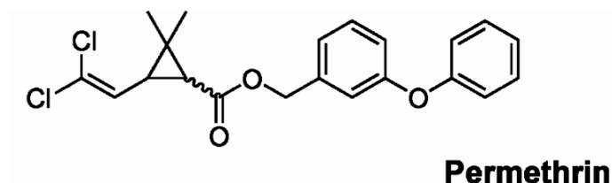
Figure 1. Chemical structure of permethrin
