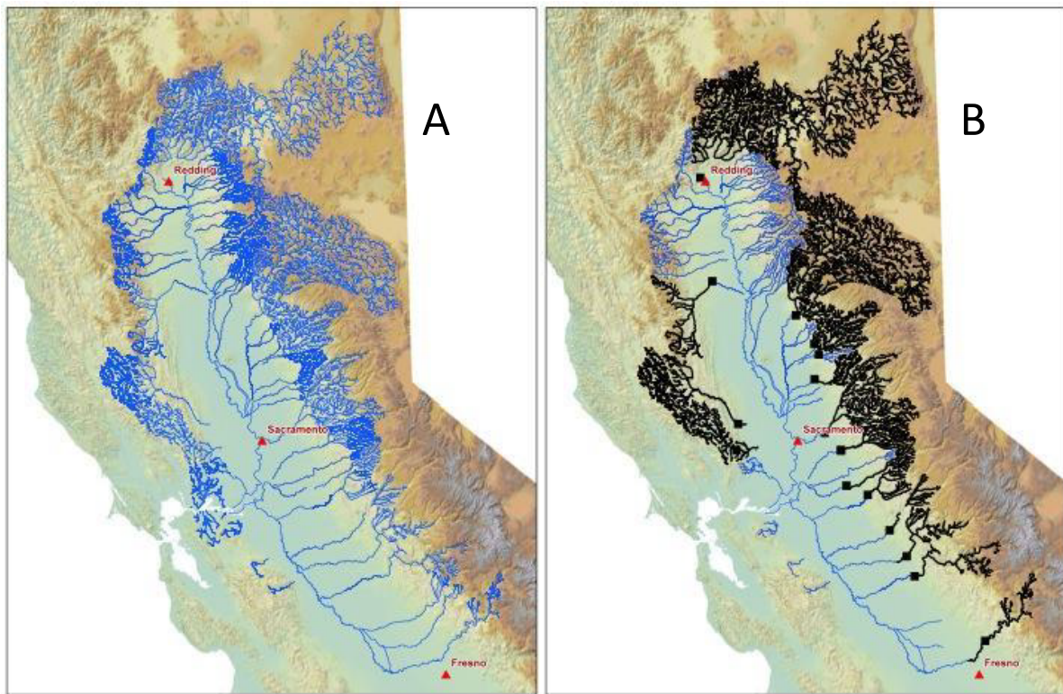
Figure 5 Historical habitat accessible to salmonids ( A , in blue) and lost upstream habitat ( B , in black) from construction of impassable dams (black squares). ( B , in blue) Remaining anadromous habitat for multiple life stages of salmon is largely confined to the valley floor. Modified from Lindley et al. (2016).
