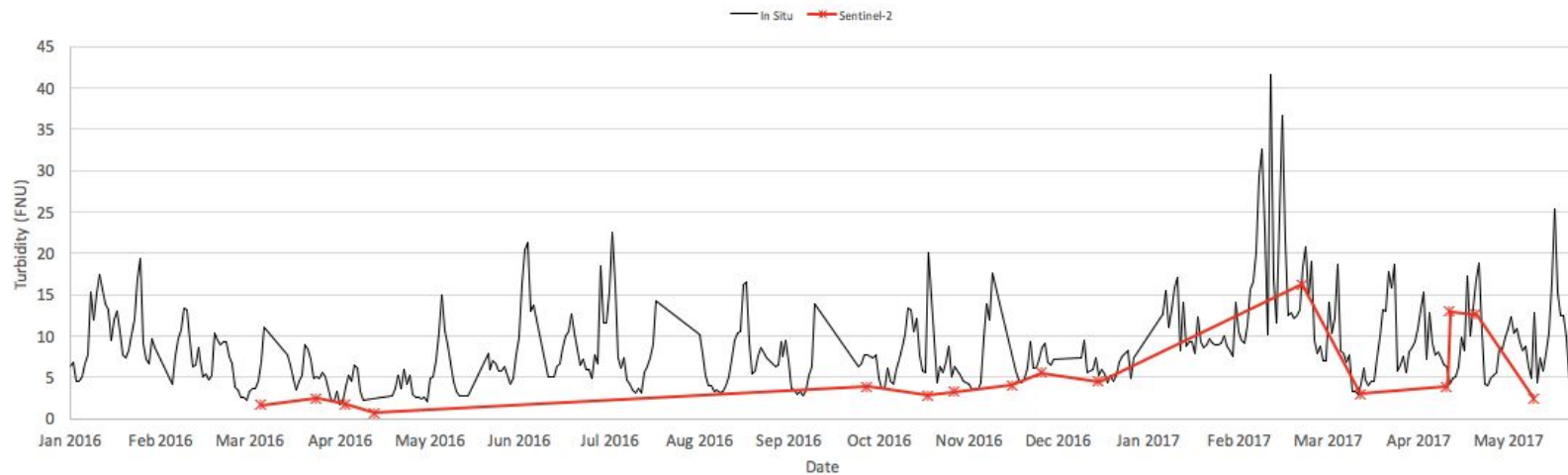
Alcatraz Station vs Sentinel-2
