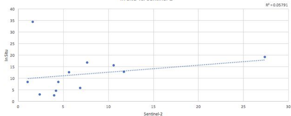
In Situ vs. Sentinel-2
