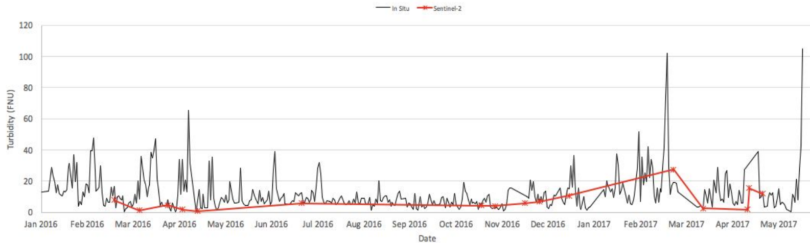
In Situ and Sentinel-2 Data for SF Pier USGS Station
