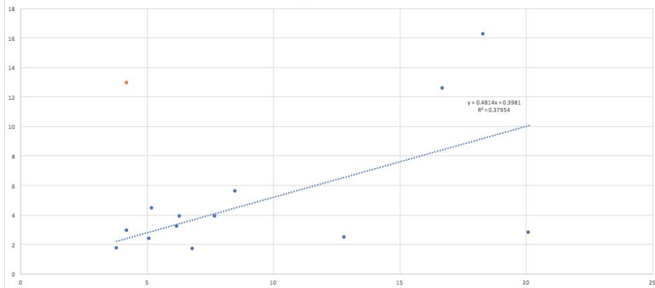
Alcatraz Station vs Sentinel-2
