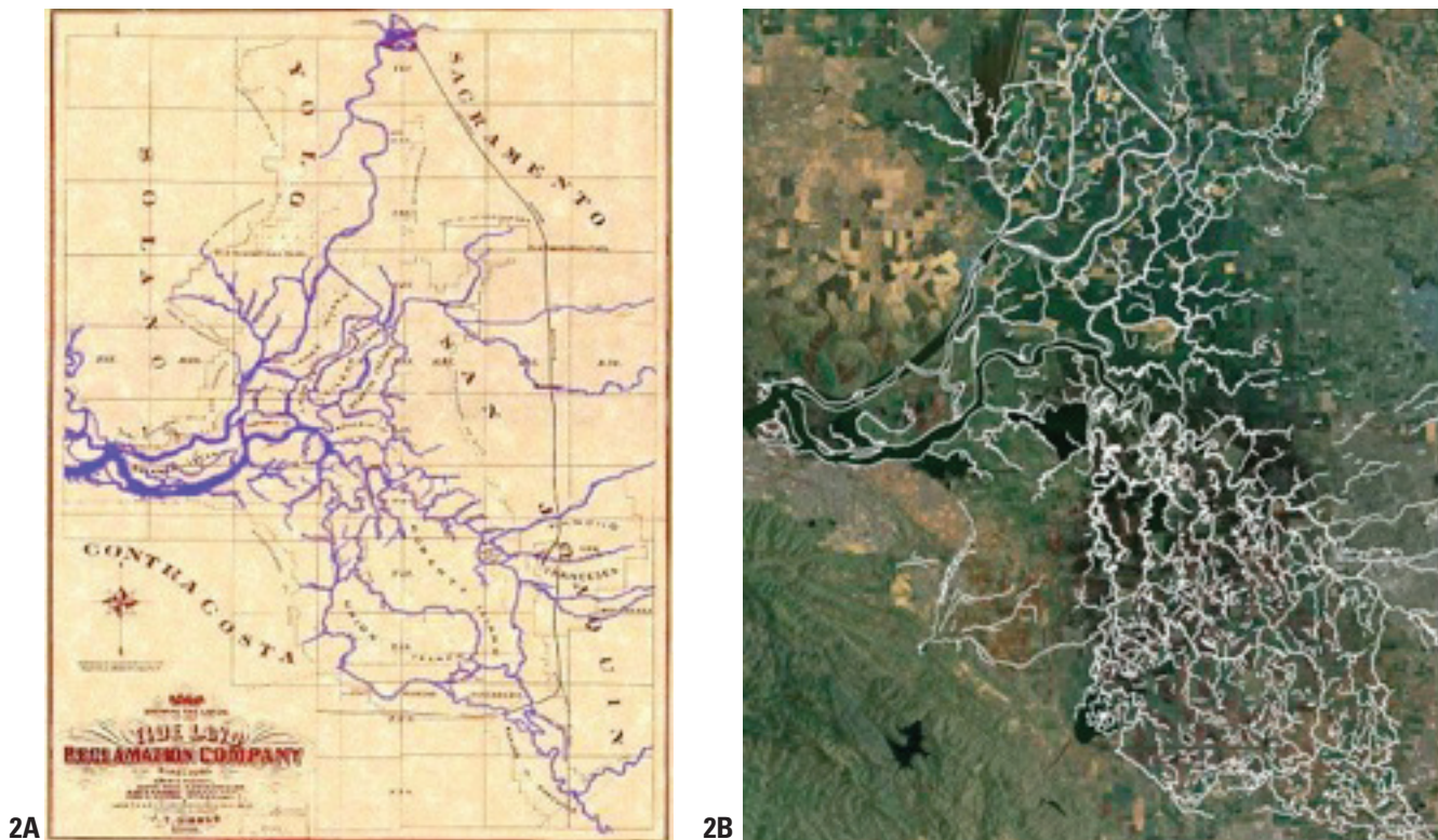
Figure 2 The Delta in the 19th century. Map 2A shows the highly complex pattern of the main river channels through the Delta (ca. 1860) while map 2B shows a re-creation of the complex marsh distributary system that once existed, especially in the south Delta. Source: Chris Enright, DWR, using Atwater data.
