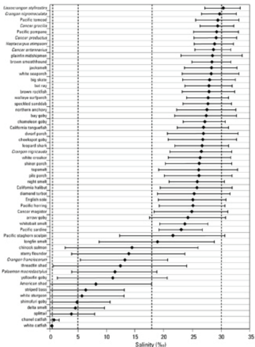
Figure 5 Mean salinity (ppt) \pm SD for the 54 most common species of fish, shrimp, and crabs collected during CDFG's Bay Study, 1980 to 1995. Source: Hieb and Fleming (1999). All species are native except chameleon goby, threadfin shad, P. macrodactylus , yellowfin goby, American shad, striped bass, shimofuri goby, channel catfish, and white catfish. The ranges shown here presumably represent optimal salinities; most species, especially those with mean salinities of <15 ppt, can be found within wider total ranges. The vertical dotted lines group the species into groups based on salinities, from left to right: (1) Delta, (2) Delta + Suisun Bay + Suisun Marsh, (3) San Francisco Bay, and (4) Pacific Ocean.
