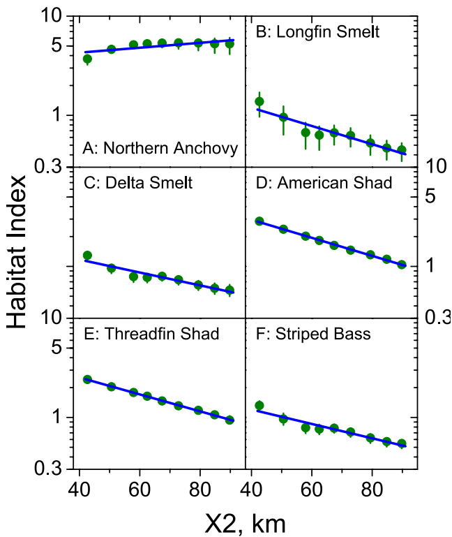
Figure 7 Examples of relationships between X_2 and habitat indices. These are for catch per trawl in the Fall Midwater Trawl Survey with salinity averaged through the water column. Each point is the volume by salinity bin, weighted by the resource selection function (Figure 6). Error bars are ranges of each habitat index determined from bootstrap sampling ( N = 25 ) of the raw data in producing the resource selection functions. Lines are least-squares fit to the log-transformed data.
