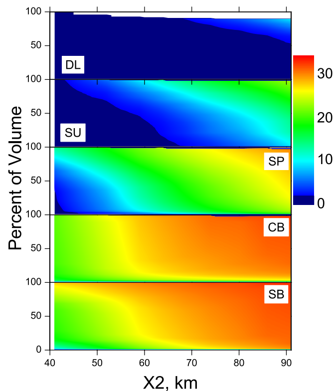
Figure 4 Volume in each region (as percent of the maximum total volume in that region) by X_2 with contours indicating depth-averaged salinity. Regions are from northeast to southwest: Delta (DL), Suisun Bay (SU), San Pablo Bay (SP), and Central (CB) and South (SB) San Francisco bays.
