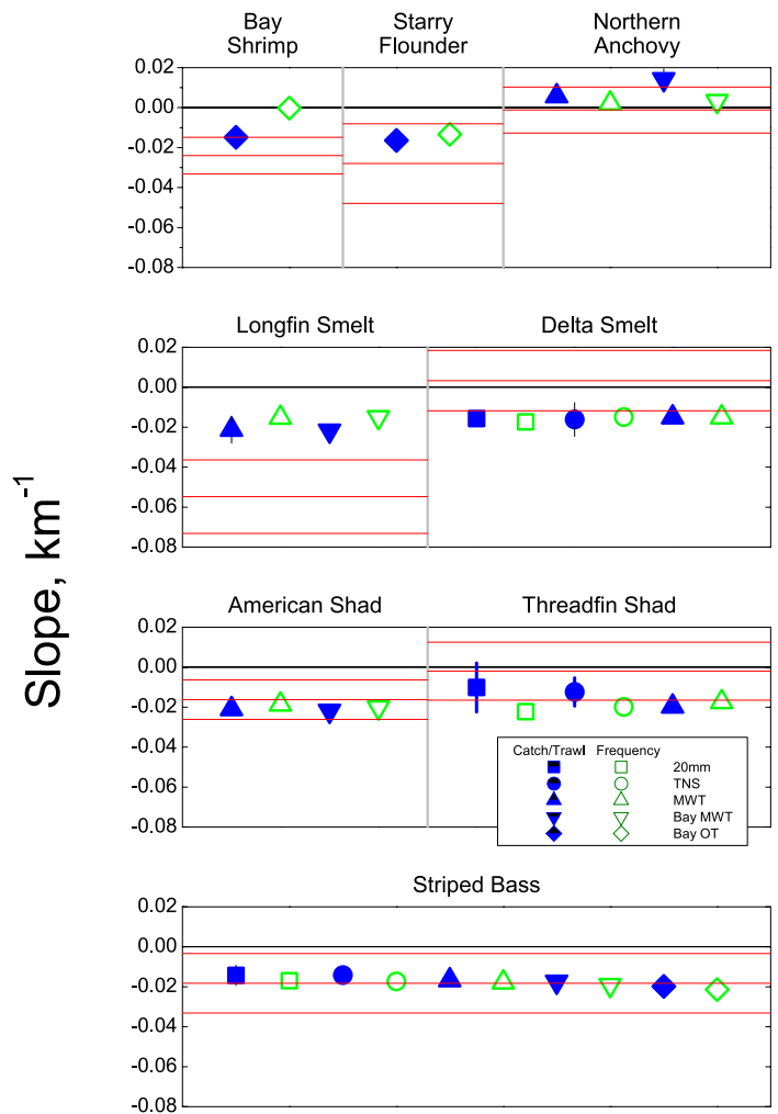
Figure 8 Slopes of relationships between habitat indices based on catch per trawl (blue filled symbols) or frequency of occurrence (green open symbols) vs. X_2 , from sampling programs indicated by shapes of symbols. The values for catch per trawl from the Fall Midwater Trawl Survey (filled triangles) are the slopes of the lines in Figure 7. Habitat indices were determined by weighting the volume in each salinity interval by the resource selection functions in Figure 6, then calculating total weighted habitat volume for each of the nine steady flows. Confidence limits for slopes of habitat vs. X_2 are contained within the symbols except where shown. Red horizontal lines indicate slopes of abundance- X_2 relationships with 95% confidence intervals (Kimmerer et al. 2009).
