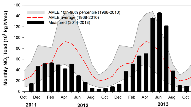
Figure 4. Monthly \text{NO}_3^- loads ( \times 10^6 kg N) and uncertainty from sensor measured values from November 2011 to November 2013. The dashed line is the monthly LOADEST average from 1968 to 2010, and the shaded area represents the 10th and 90th percentiles over the same period.
