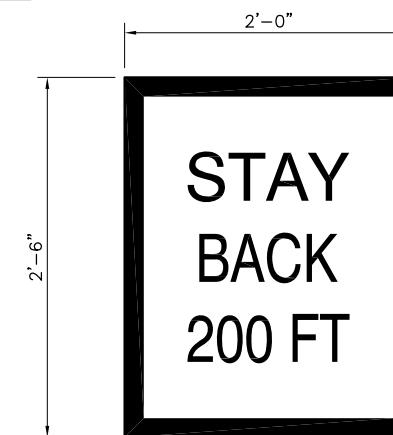
8 ELECTRONIC MESSAGE SIGN C19 SCALE: NONE C47
