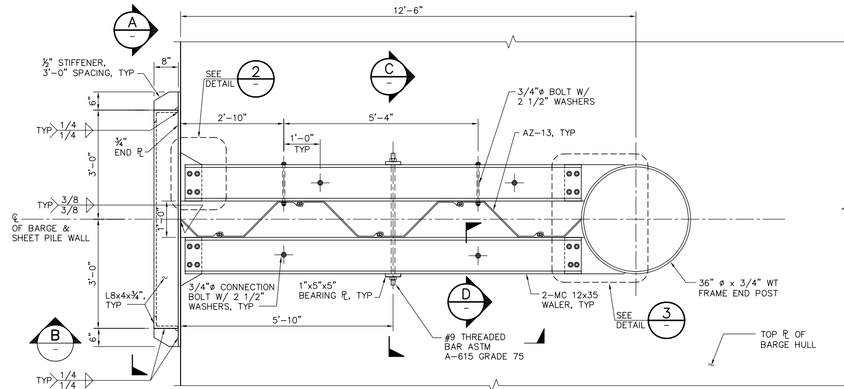
PLAN
