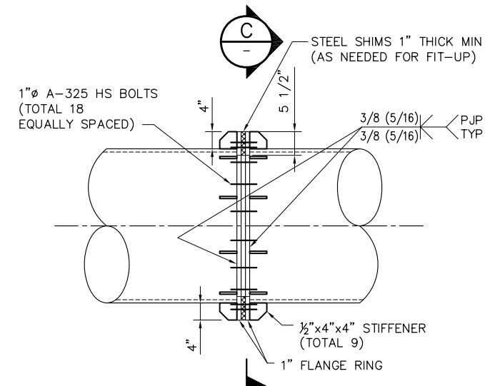
3 UHMW HDPE THRUST BEARING C17 SCALE: 3/4" = 1'-0" C45, C59
