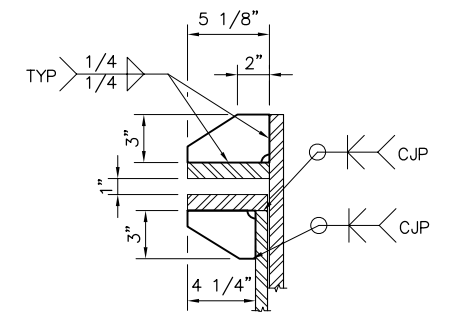
3 DETAIL NTS
