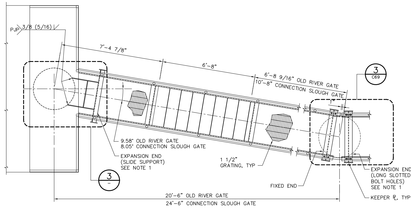
PLAN 1 DETAIL C12 SCALE: 1/2" = 1'-0" C40
