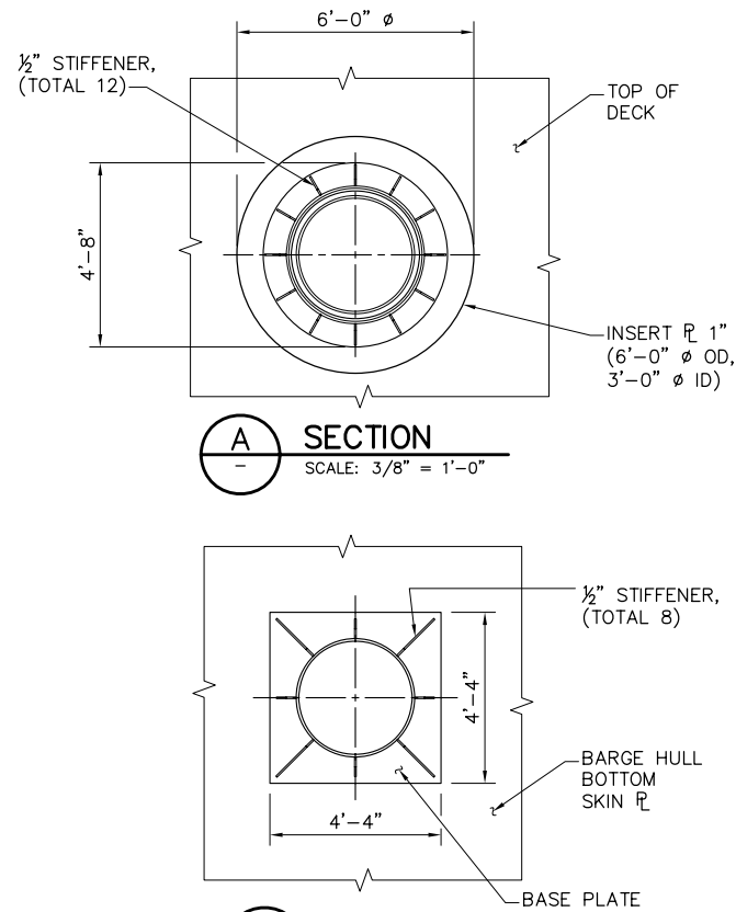
2 FRAME CONNECTION C17 SCALE: 3/4" = 1'-0" C59
