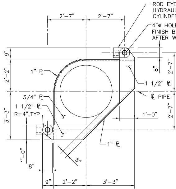
2 GATE YOKE DETAIL SCALE: 1/2" = 1'-0"
