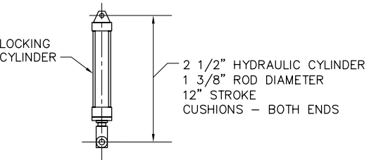
8 LOCKING CYLINDER DETAIL SCALE: 1" = 1'-0"
