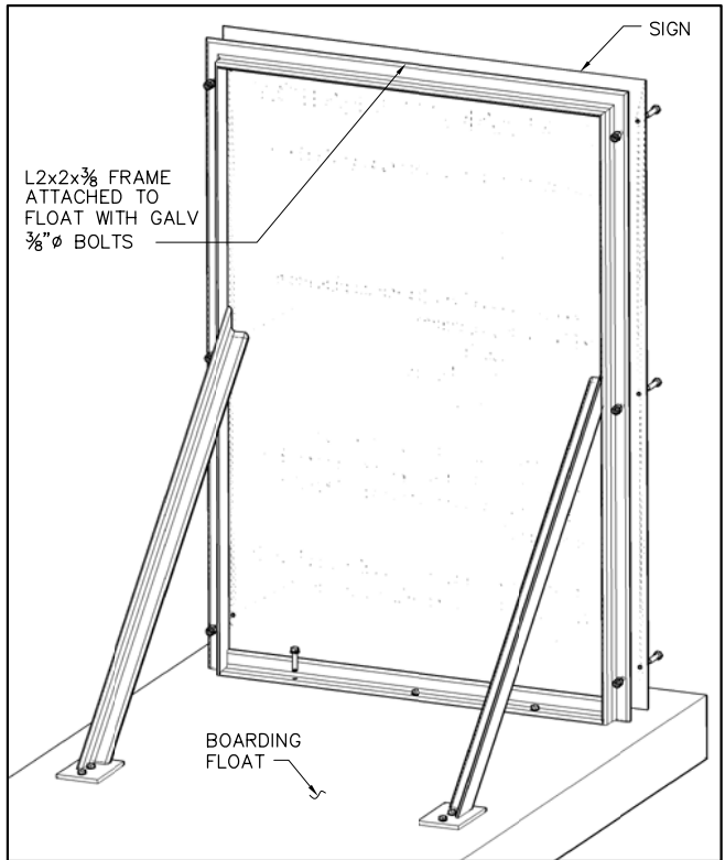
6 BOAT RAMP DOCK SIGN C19 SCALE: NONE C47
