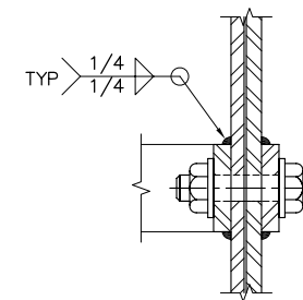
2 DETAIL NTS
