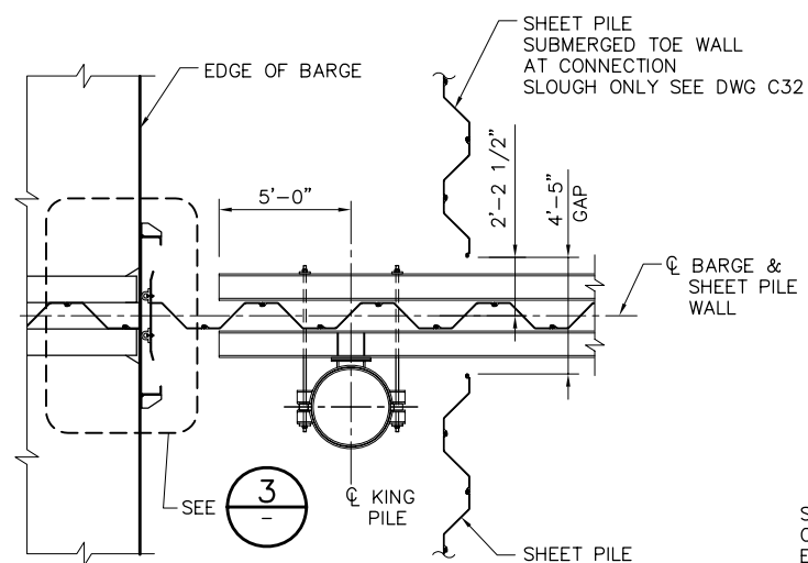
PLAN DETAIL SCALE: 1/4" = 1'-0"
