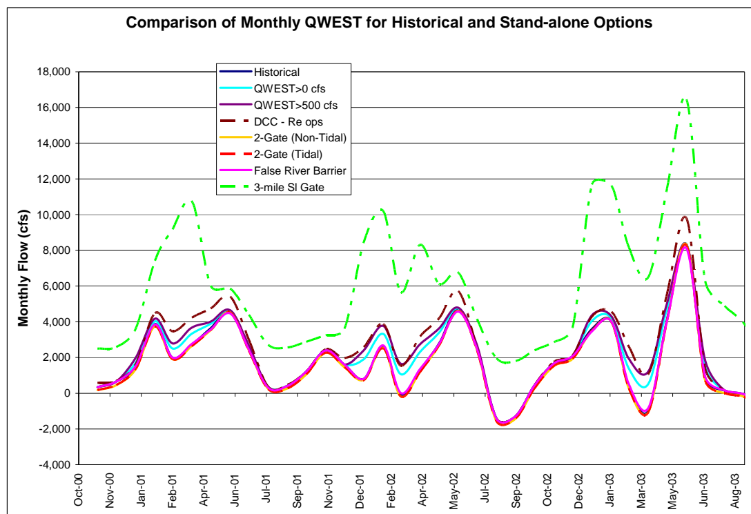
Figure K-6: Comparison of monthly QWEST flow from stand-alone near-term options and the baseline simulation
