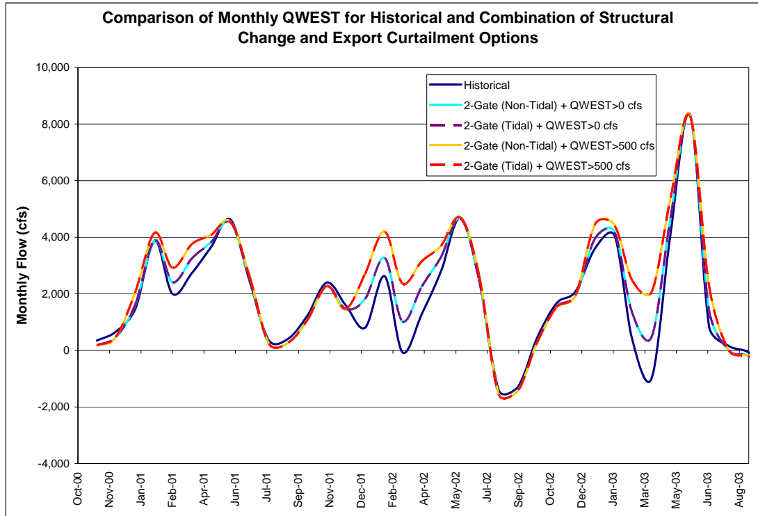
Figure K-10: Comparison of monthly QWEST flow from combinations of structural changes and export curtailments and the baseline simulation
