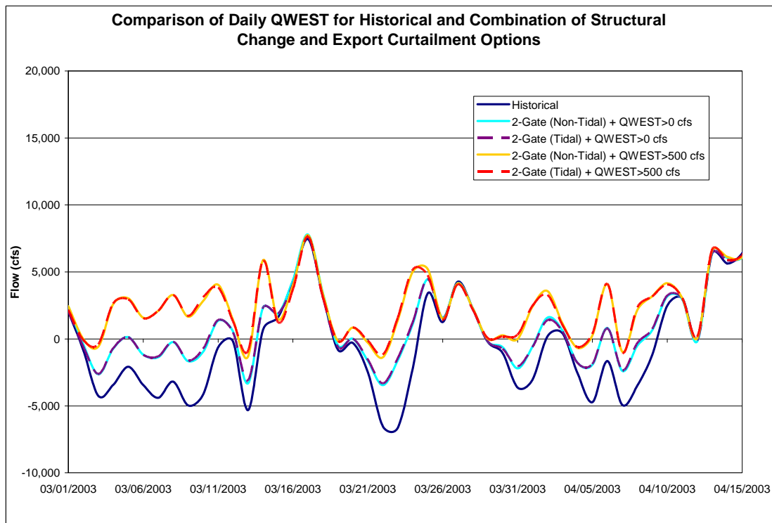
Figure K-11: Comparison of daily QWEST flow from combinations of structural changes and export curtailments and the baseline simulation during March 1, 2003 to April 15, 2003
