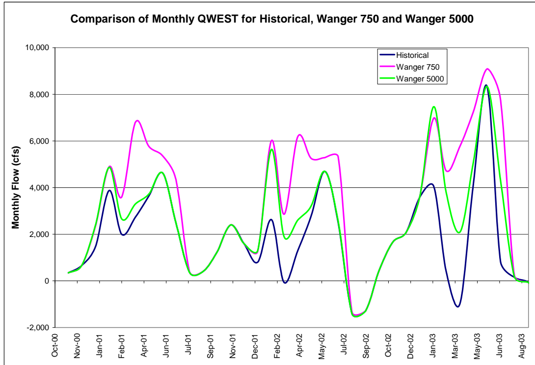
Figure K-4: Comparison of average monthly QWEST flow from baseline, Wanger 750 and Wanger 5000 scenarios
