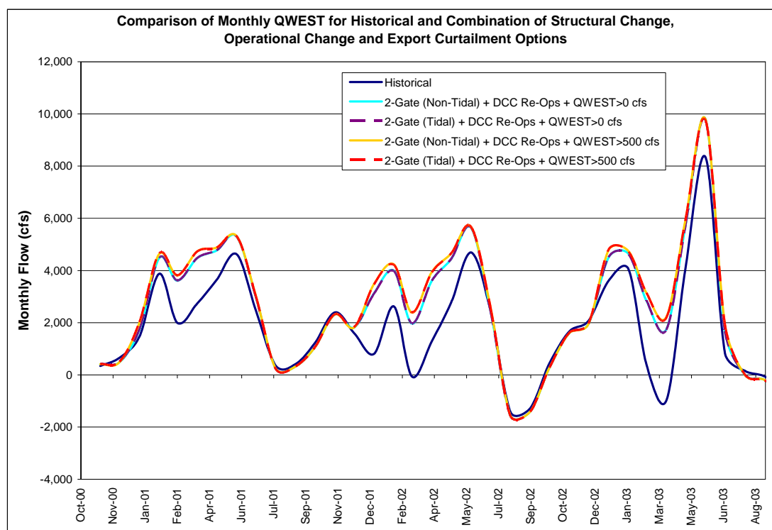
Figure K-14: Comparison of monthly QWEST flow from combinations of structural changes, operational changes and export curtailments and the baseline simulation
