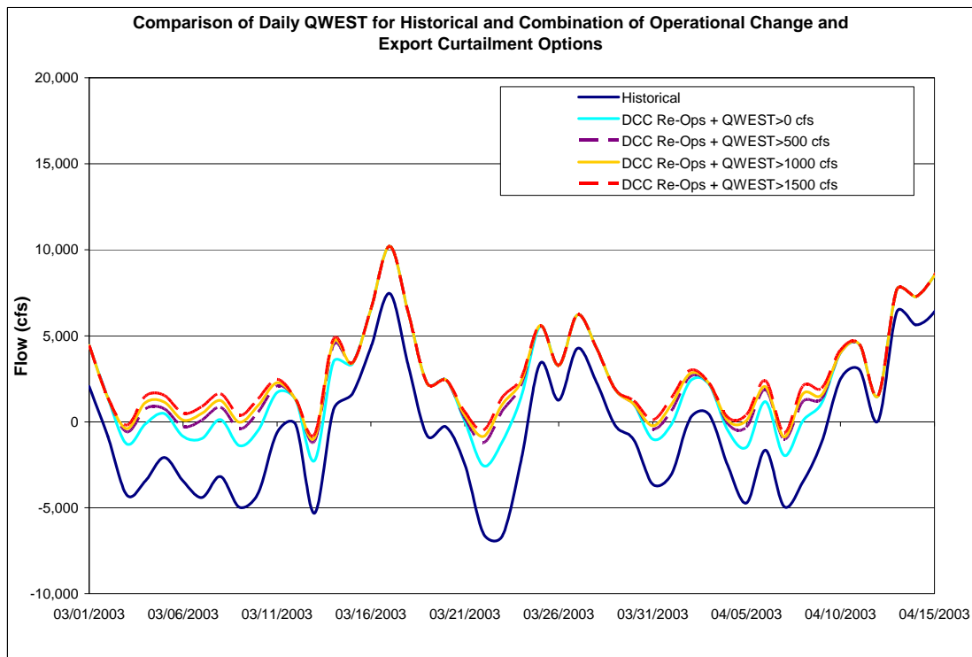
Figure K-9: Comparison of daily QWEST flow from combinations of operational changes and export curtailments and the baseline simulation during March 1, 2003 to April 15, 2003
