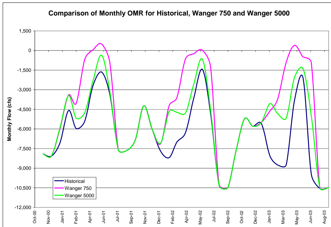
Figure K-3: Comparison of average monthly combined Old and Middle River flow from baseline, Wanger 750 and Wanger 5000 scenarios
