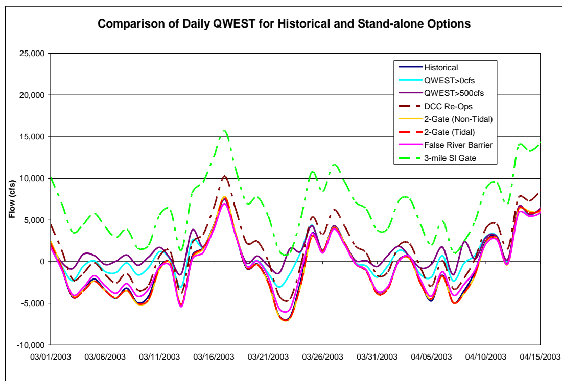
Figure K-7: Comparison of daily QWEST flow from stand-alone near-term options and the baseline simulation during March 1, 2003 to April 15, 2003
