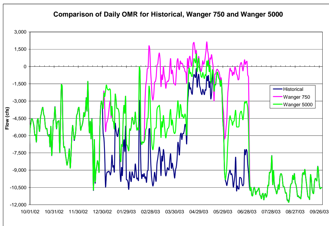
Figure K-2: Comparison of average daily combined Old and Middle River flow for WY 2003 from baseline, Wanger 750 and Wanger 5000 scenarios
