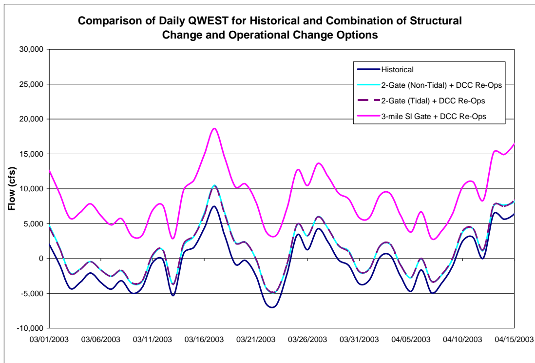
Figure K-13: Comparison of daily QWEST flow from combinations of structural changes and operational changes and the baseline simulation during March 1, 2003 to April 15, 2003
