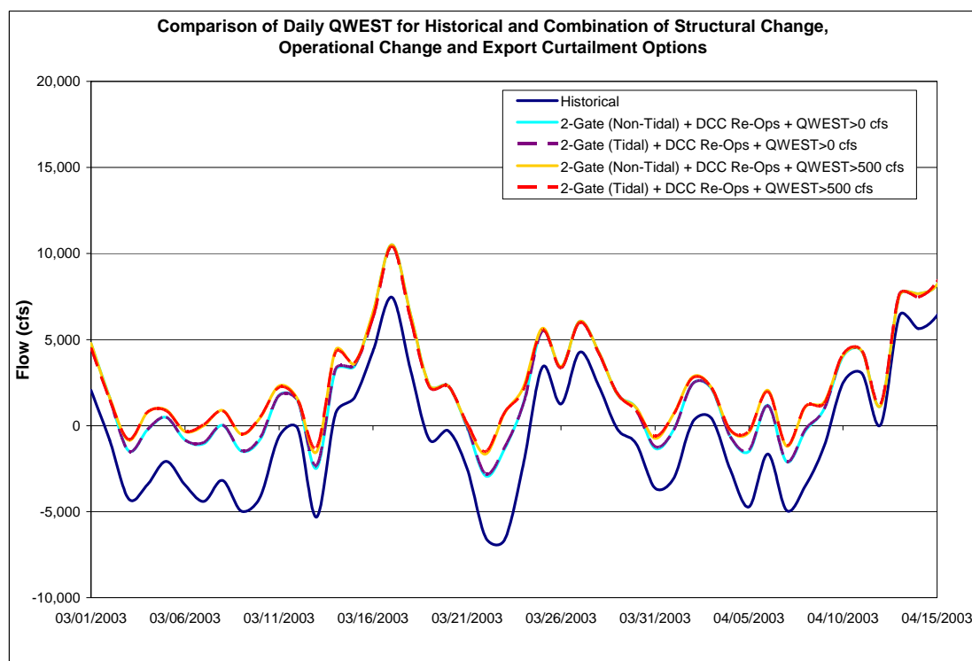
Figure K-15: Comparison of daily QWEST flow from combinations of structural changes, operational changes and export curtailments and the baseline simulation during March 1, 2003 to April 15, 2003
