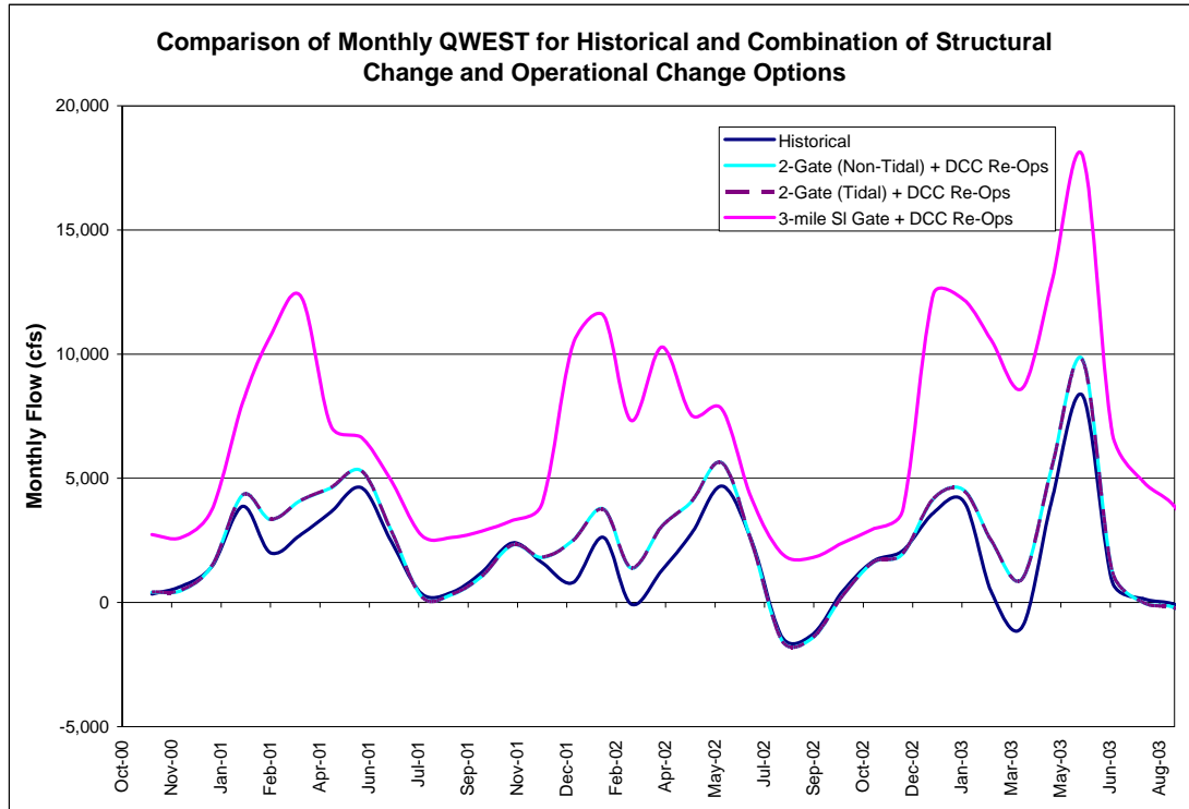
Figure K-12: Comparison of monthly QWEST flow from combinations of structural changes and operational changes and the baseline simulation
