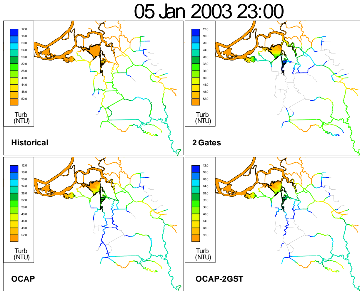
Figure 5 Simulated turbidity for historical conditions, OCAP operations, 2-gate scenario, and OCAP operations with 2-gate start time (OCAP-2GST) on 05 Jan 2003 at 23:00.
