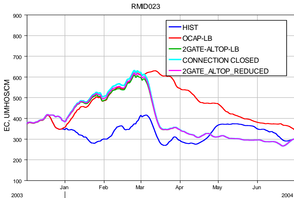
Figure 17 Tidally averaged EC at RMD023 for the 2003-2004 simulation period for HIST, OCAP-LB and 2GATE-ALTOP-LB, CONNECTION CLOSED and 2GATE_ALTOP_REDUCED simulations.
