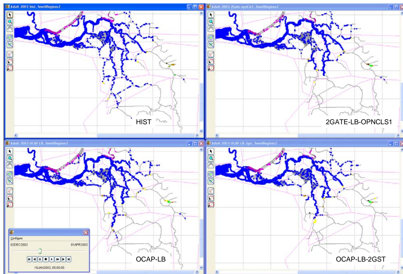
Figure 5-2. Adult Delta Smelt Particle Distributions for Historical Conditions (HIST), OCAP Operations (OCAP-LB), and 2-Gates Scenario (2GATE_LB-OPNCLS1). The Difference between OCAP and OCAP with 2-GATE is the Comparison of Lower Left with Upper Right Figures
