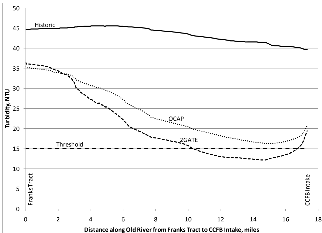
Figure 5-1. Longitudinal Profile of Modeled Turbidity along Old River from Franks Tract to Clifton Court Forebay Showing the Amount of the Old River Channel with Reduced Turbidity from OCAP and the 2-Gates Compared to Historical Conditions
