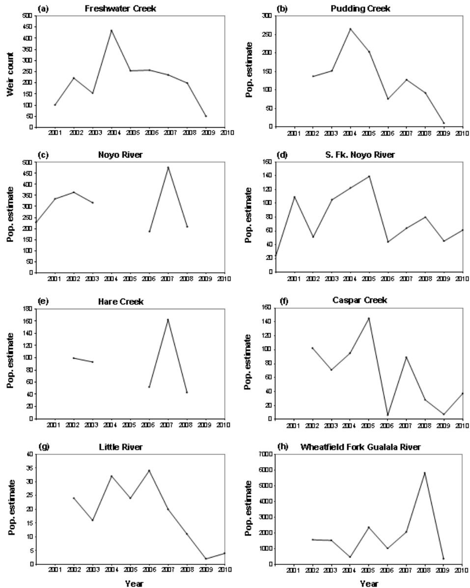
Figure 13. Population estimates, indices, weir counts and dive counts for NC-Steelhead. Populations are winter-run unless otherwise noted. Note: for winter-run, year 2010 indicates the 2009-2010 spawning season. For summer-run, year is the year of survey.
