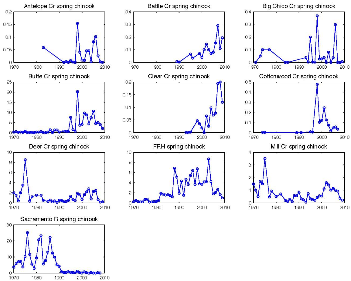
Figure 20. Time series of escapement for Central Valley spring-run Chinook salmon populations. Y axis is in thousands of fish.
