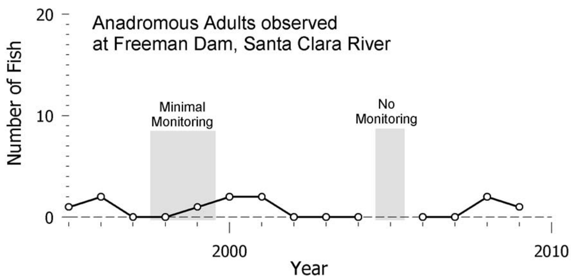
Figure 15. Anadromous O. mykiss observed in the Santa Ynez River system, by staff of the Cachuma Conservation Release Board; and at the fish-passage facility for the Freeman Dam on the Santa Clara River, by staff of the United Water District. Numbers are incomplete counts, unadjusted for observation probabilities; see text for details.
