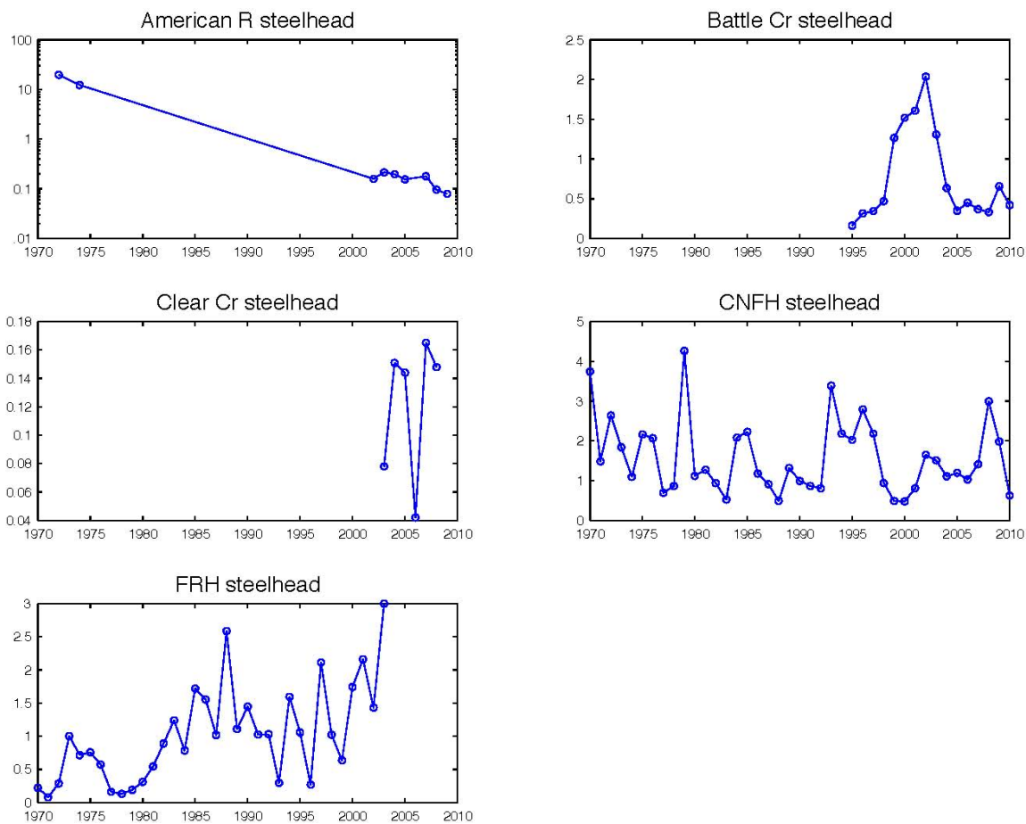
Figure 21. Time series of escapement for Central Valley steelhead populations. Y axis is in thousands of fish. Note that the y-axis of plot for American River steelhead is on a logarithmic scale.
