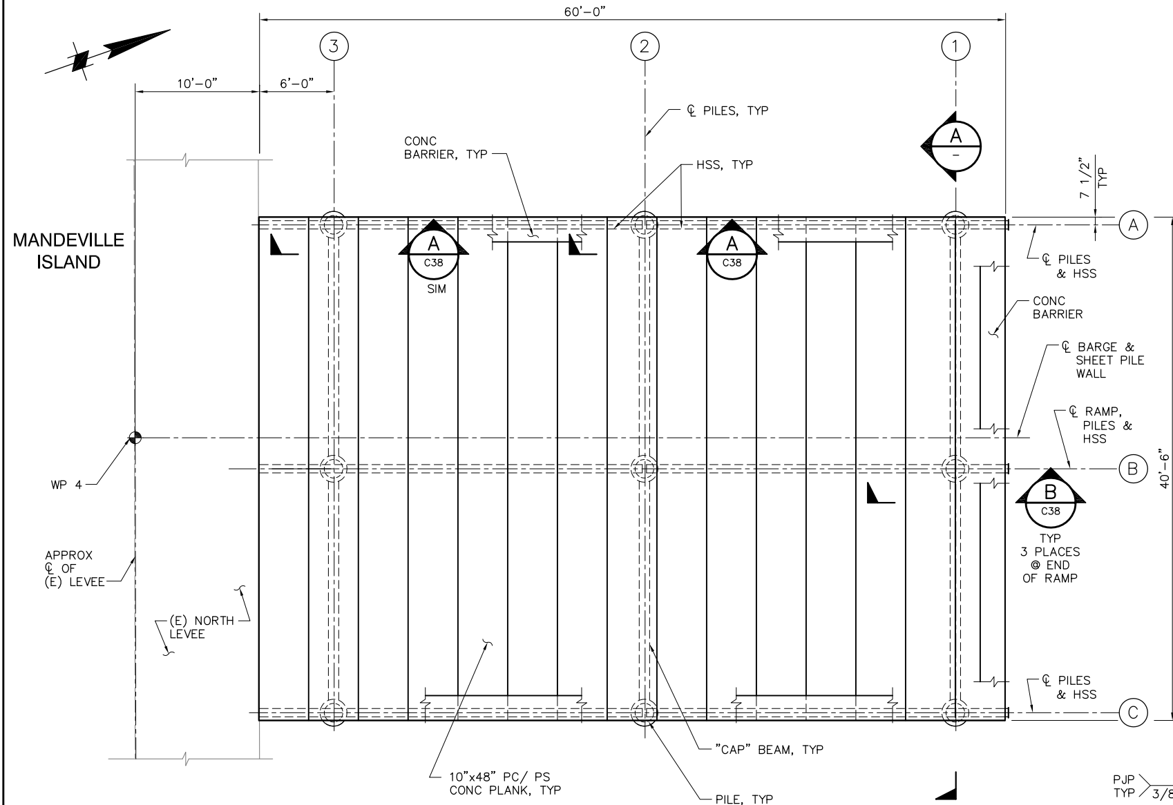
1 DETAIL SCALE: 3/16" = 1'-0"
