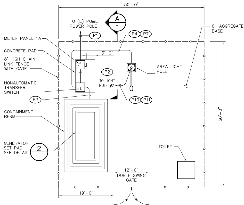
1 UTILITY YARD C13 SCALE: 1/8"=1'-0" C41
