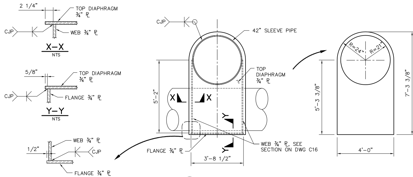
1 SLEEVE CONNECTION DETAIL SCALE: 1/2" = 1'-0"
