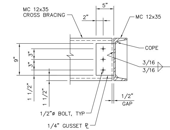
2 TYPICAL GUSSET CONNECTION DETAIL SCALE: 1 1/2" = 1'-0"
