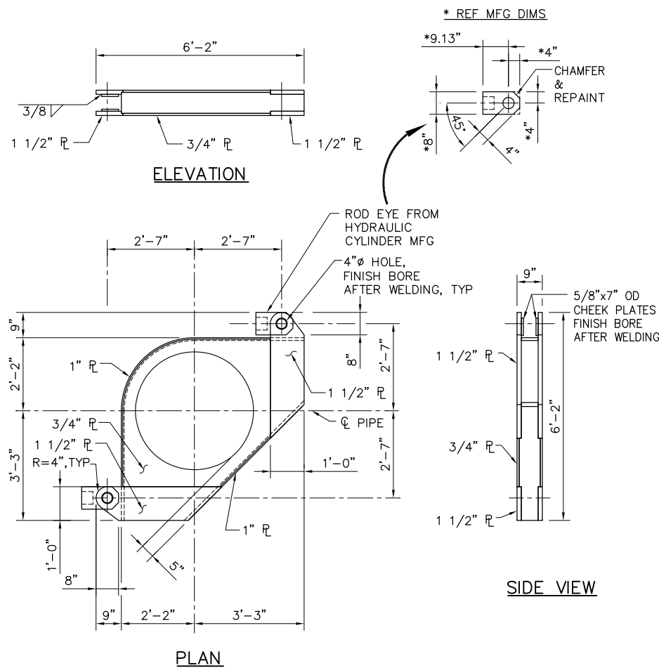
2 GATE YOKE DETAIL C44 SCALE: 1/2" = 1'-0"
