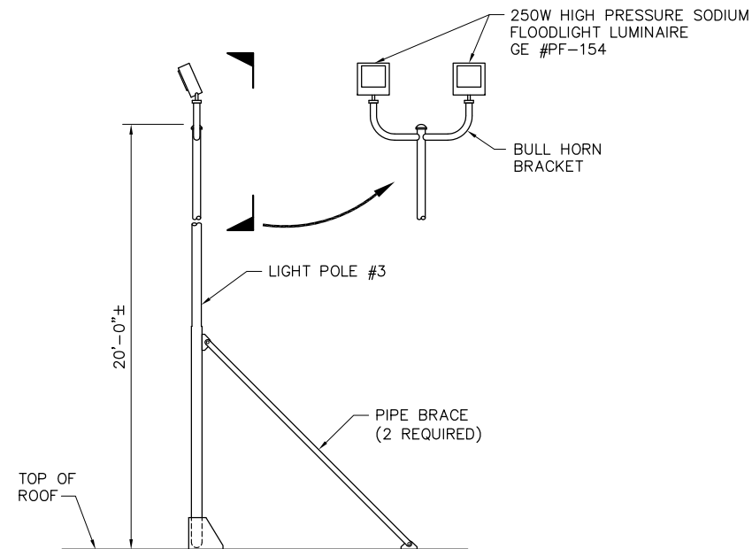
2 FOLD-DOWN LIGHT POLE DETAIL C13 NTS
