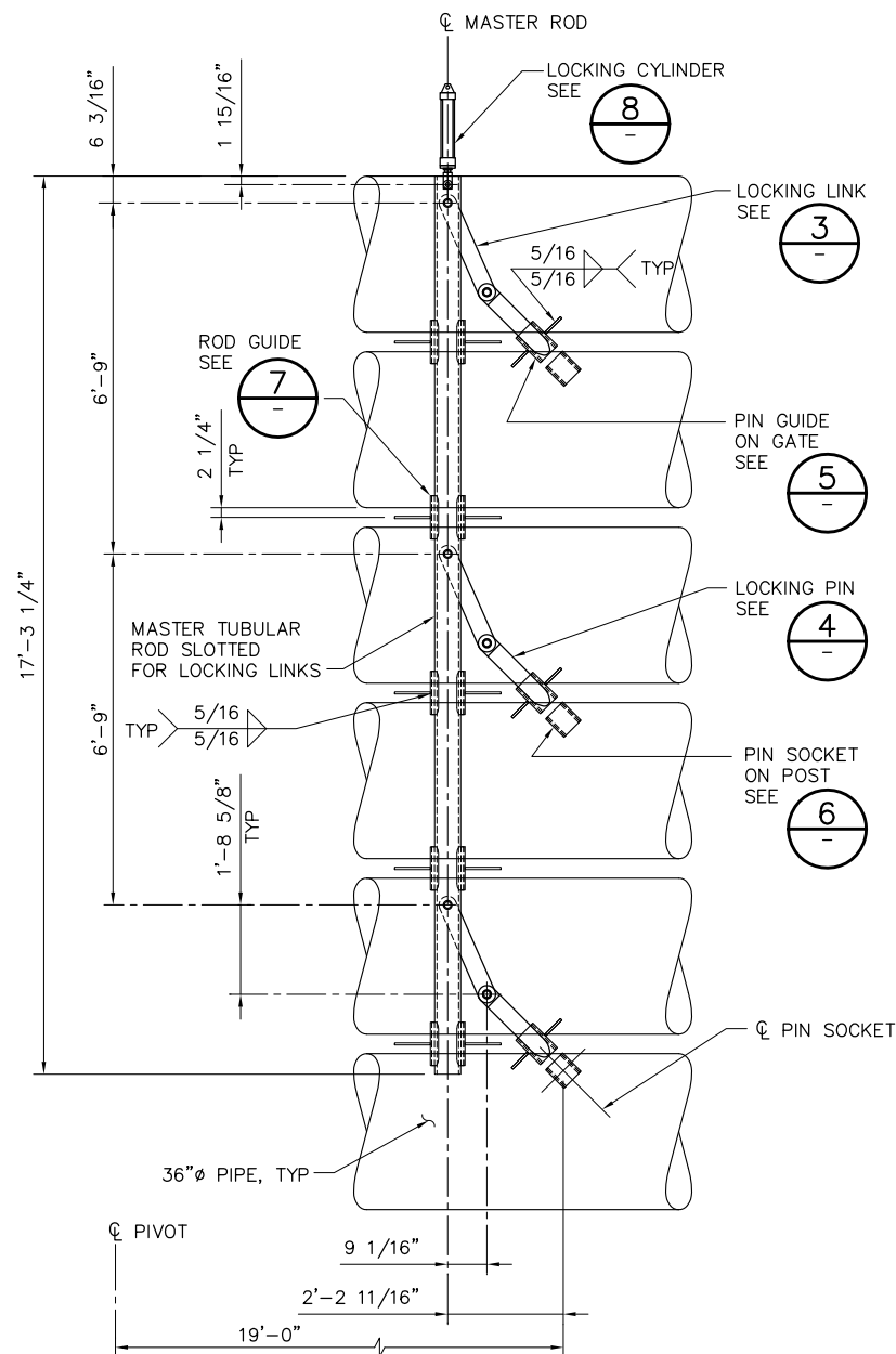
1 GATE OPEN LOCK (UNLOCKED) DETAIL C43 SCALE: 1/2" = 1'-0"
