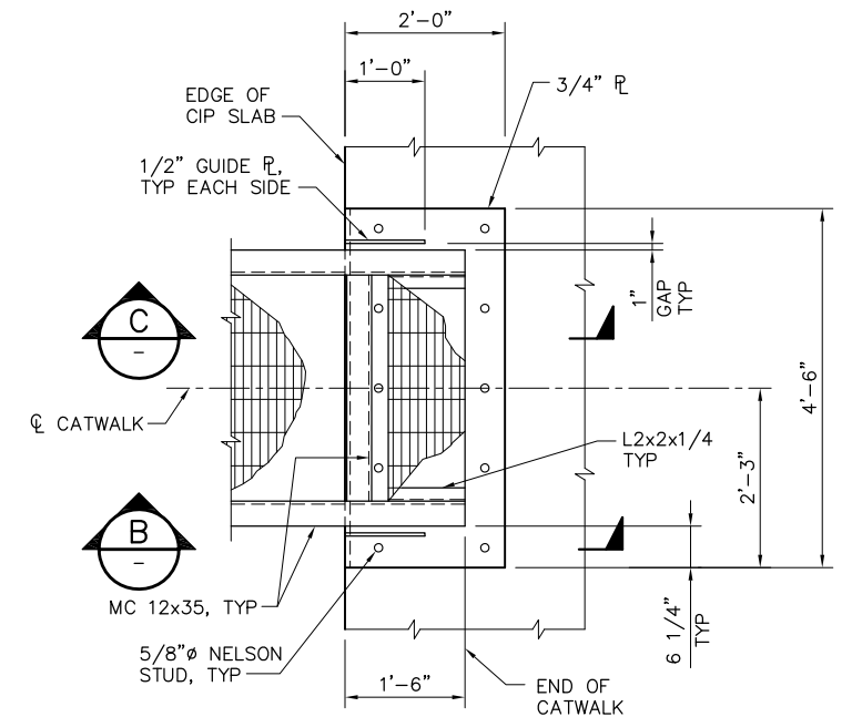
PLAN AT END OF CATWALK SCALE: 3/4" = 1'-0"
