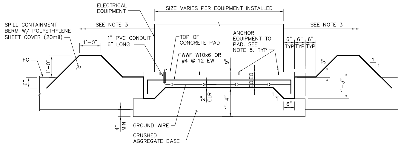
2 GENERATOR SET PAD DETAIL NTS
