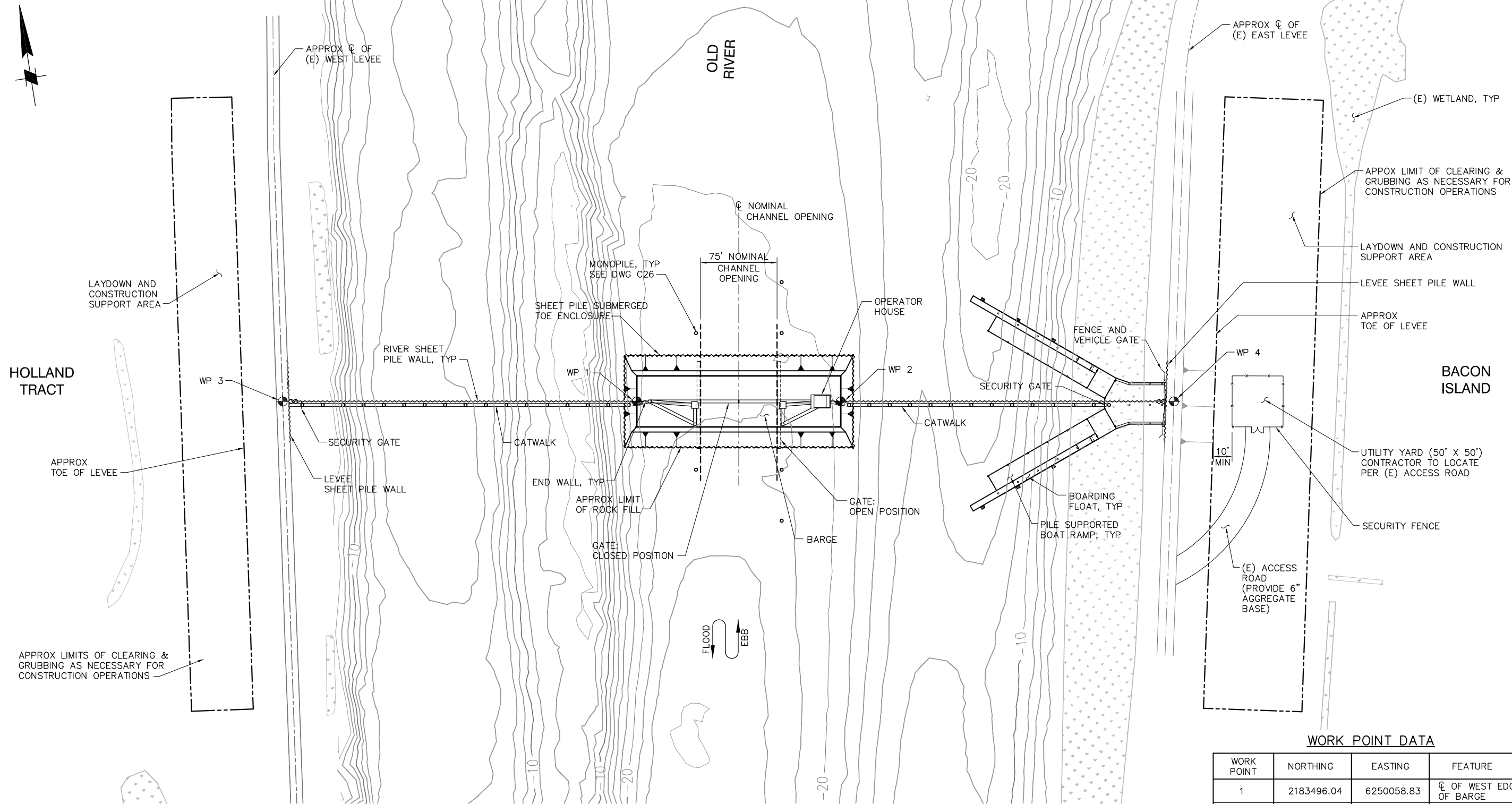
SITE PLAN SCALE: 1"= 50'
