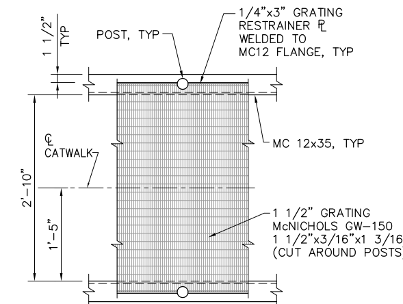
PLAN AT GRATING PLATE
