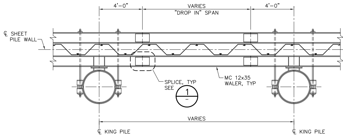
PLAN TYPICAL WALER SPLICE DETAIL (SEE NOTE 1) SCALE: 3/4" = 1'-0"
