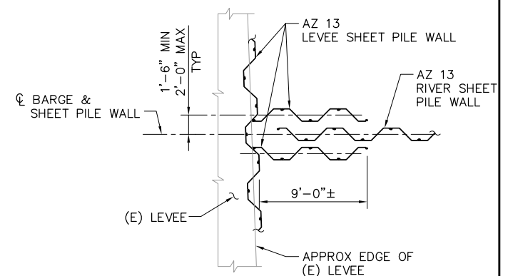
5 DETAIL SCALE: 3/16" = 1'-0"
