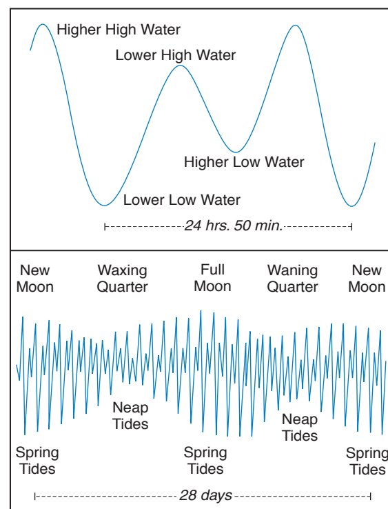
The Tides near San Francisco
