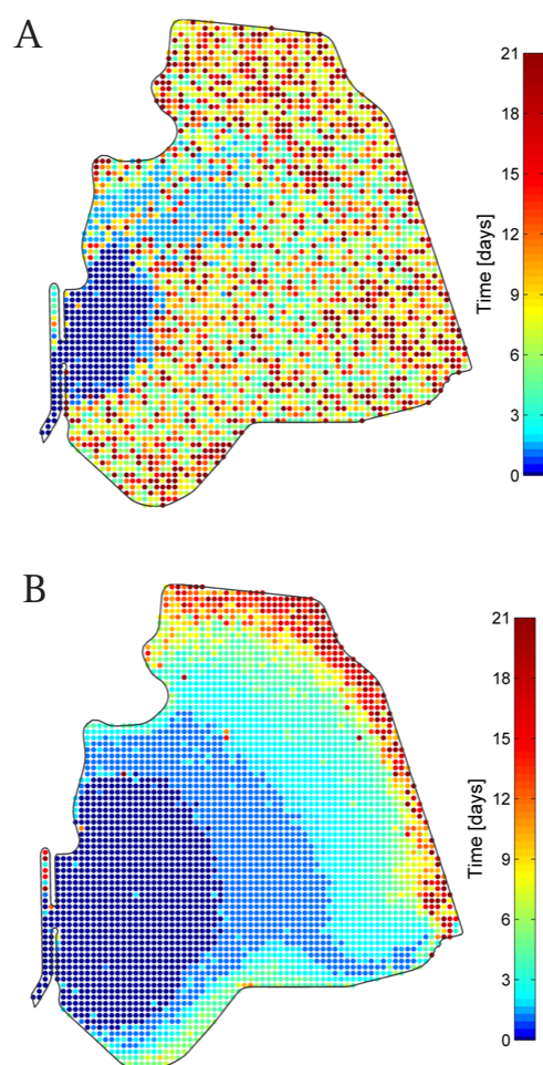
Figure 7 Predicted residence time of particles shown at the release location of each particle. (A) Particles released on June 9, 2008 at 00:00 PST during low export pumping conditions; (B) Particles released on January 10, 2009 at 00:00 PST during moderate export pumping conditions.
