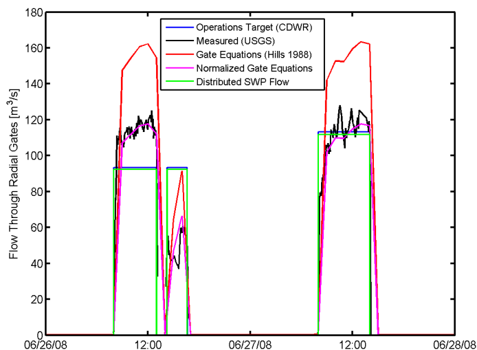
Figure 4 Flow estimates through the radial gates into CCF on June 26 and 27, 2008
