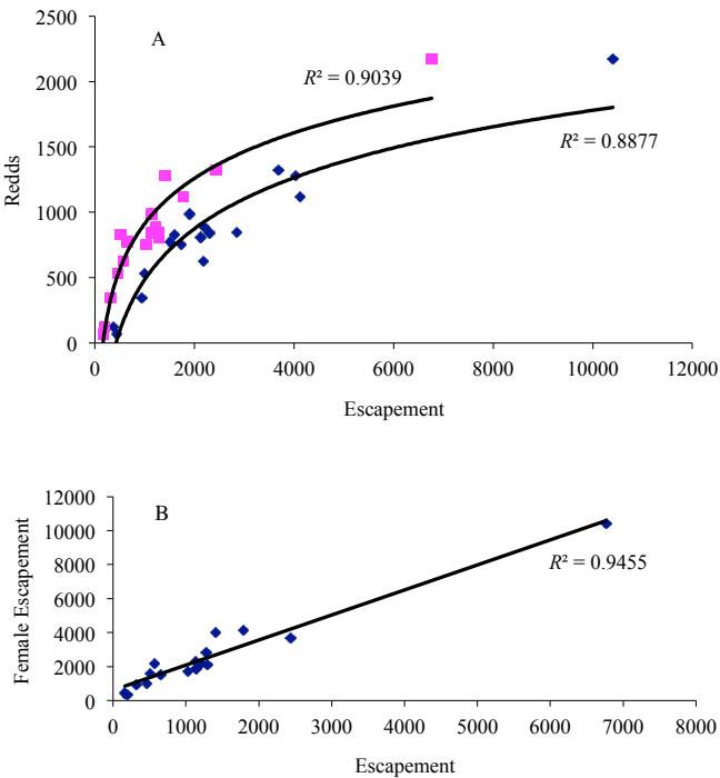
Figure 5 The relationship between (A) log estimated total escapement and estimated redds (diamond) and log total female escapement and estimated redds (square) and (B) total escapement and female escapement for the lower Mokelumne River, California (1990–2006)
