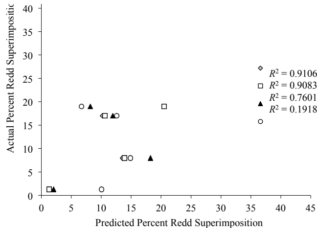
Figure 6 Regression between observed and predicted percent redd superimposition for 5 variable flow years (1991–1995) on the lower American River, California. Percent superimposition predictions were modeled using redd counts (white circles), flow (black triangles), interaction of redds and flow (white squares) and additive effects of redds and flow (gray diamonds).
