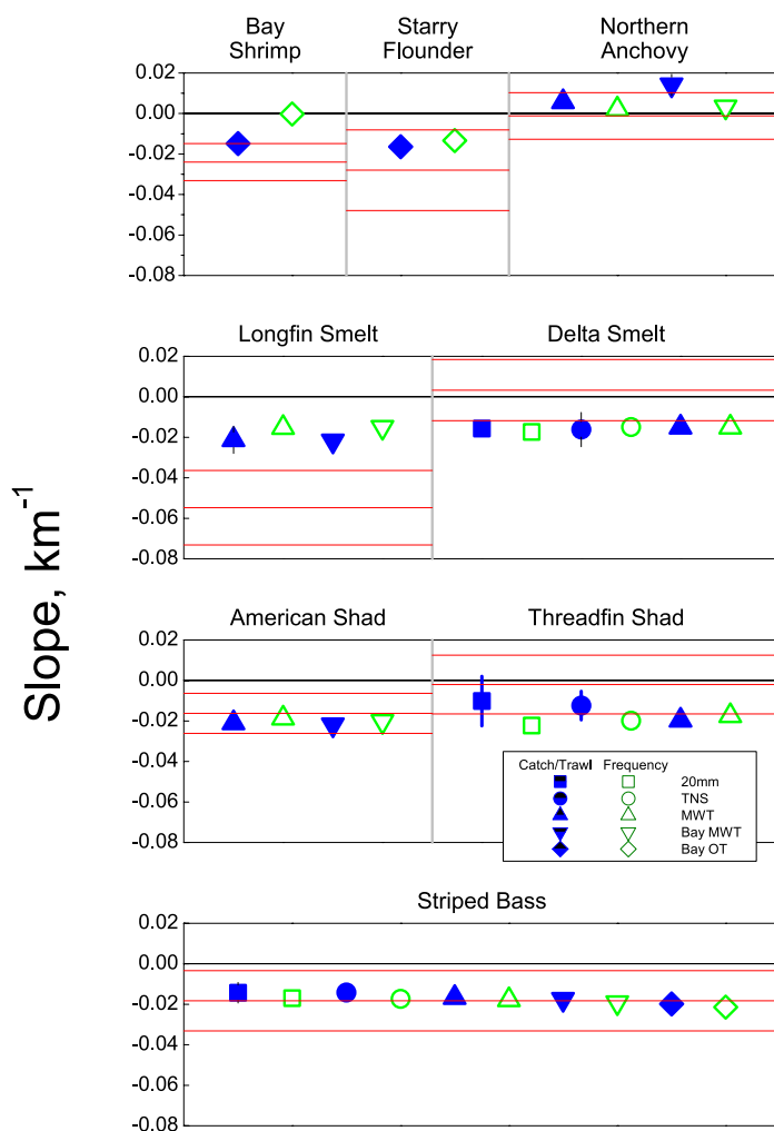
Figure 8 Slopes of relationships between habitat indices based on catch per trawl (blue filled symbols) or frequency of occurrence (green open symbols) vs. X_2 , from sampling programs indicated by shapes of symbols. The values for catch per trawl from the Fall Midwater Trawl Survey (filled triangles) are the slopes of the lines in Figure 7. Habitat indices were determined by weighting the volume in each salinity interval by the resource selection functions in Figure 6, then calculating total weighted habitat volume for each of the nine steady flows. Confidence limits for slopes of habitat vs. X_2 are contained within the symbols except where shown. Red horizontal lines indicate slopes of abundance- X_2 relationships with 95% confidence intervals (Kimmerer et al. 2009).
