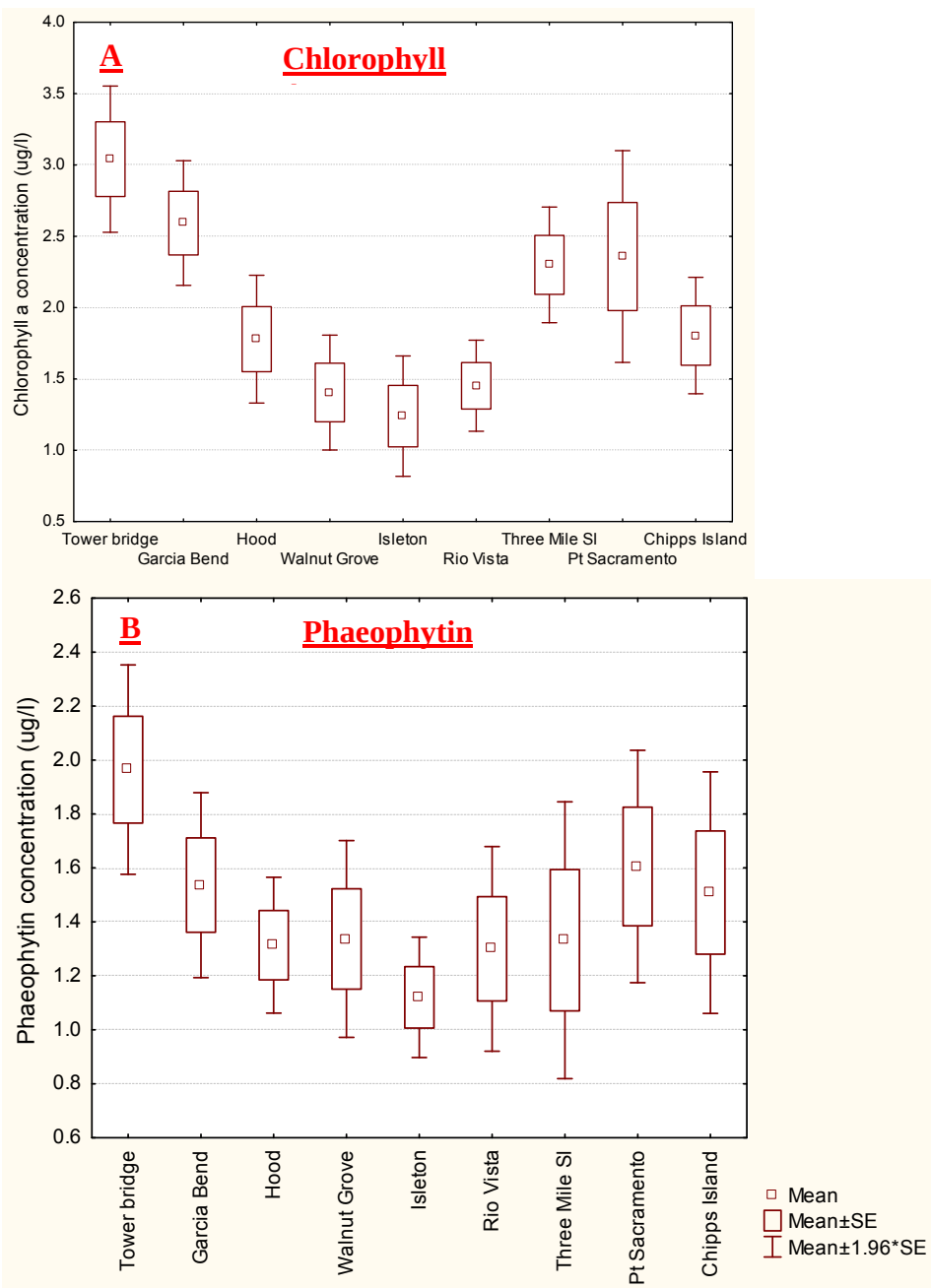
Figure 4A. Mean annual chlorophyll a concentrations in the lower Sacramento River and across the Delta to Chipps Island. B. Same values for phaeophytin.
