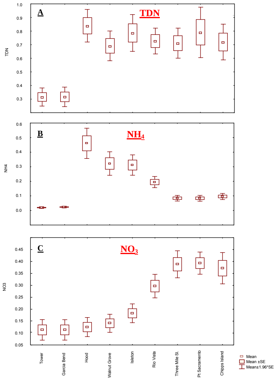
Figure 2. A . Mean annual total dissolved nitrogen (TDN) concentrations on the Sacramento River between Tower Bridge and Chipps Island. The SRWTP discharges between Garcia Bend and Hood. B and C Ammonia (NH 4 ) and nitrate (NO 3 ) concentrations over the same river reach. All nitrogen concentrations are as mg N/L
