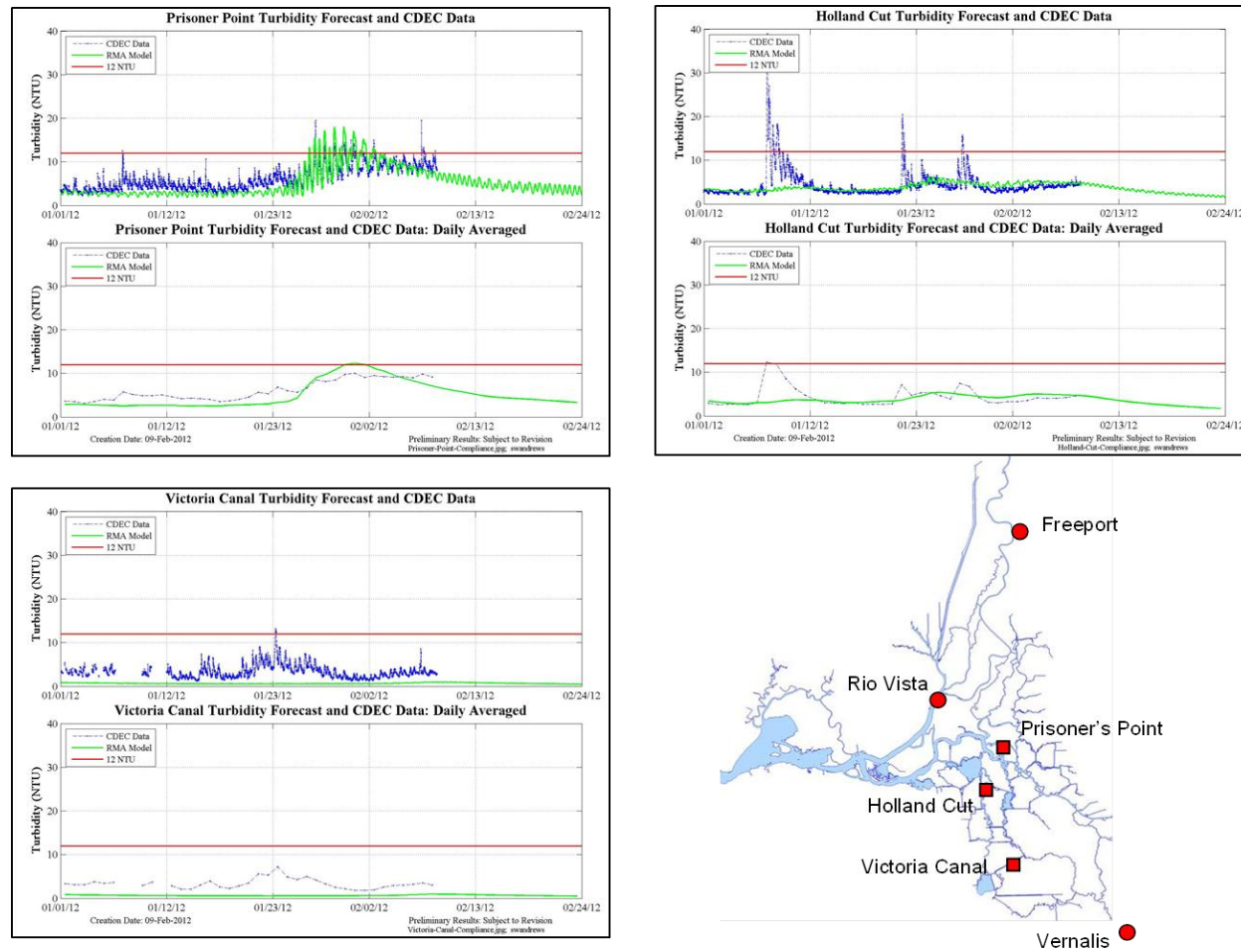
Figure 16 Modeled turbidity and data (cleaned and filled) at the three compliance locations. Both 15-min model output and data and daily averaged plots are shown. Red line illustrates the 12-NTU compliance value.
