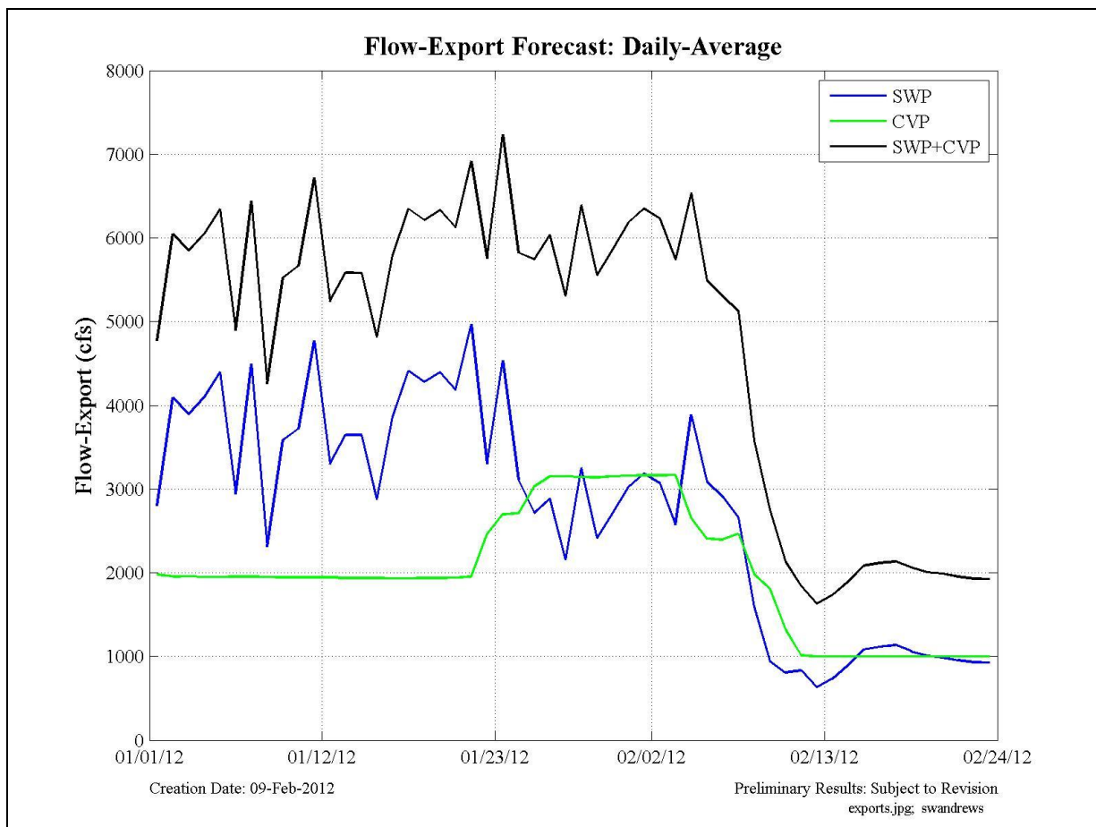
Figure 12 Historical and modeled daily-averaged exports at the SWP and CVP export locations, and the combined SWP+CVP exports.
