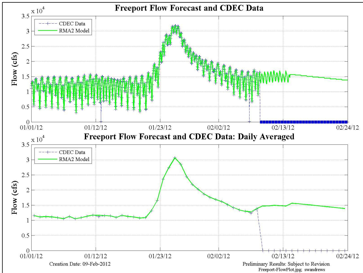
Figure 2 Freeport flow BC was compiled using CDEC data, CNRFC forecast, and then DWR DSM2 forecast. Note y-axis unit is cfs*10,000. Zero values indicate the end of data (blue).
