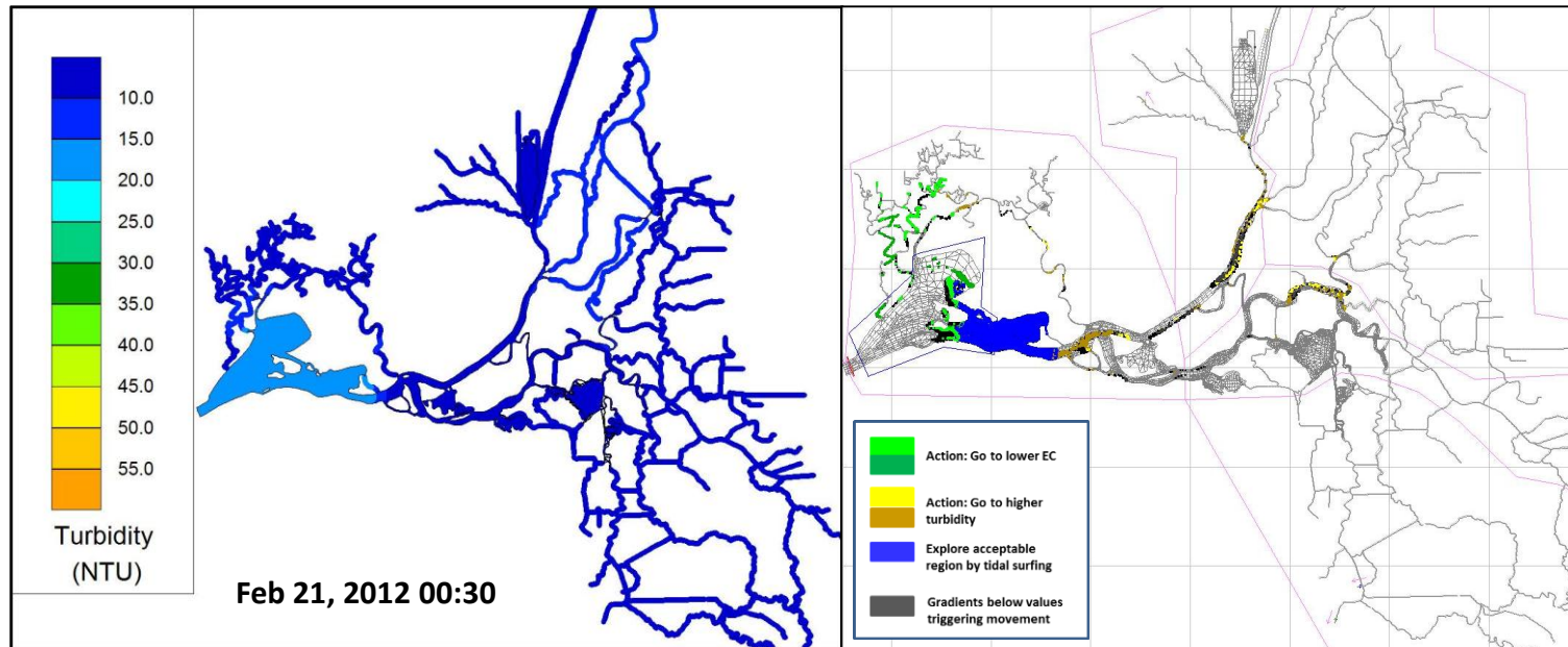
Figure 31 Turbidity contours and particle location in the RMA model grid on Feb. 21, 2012.
