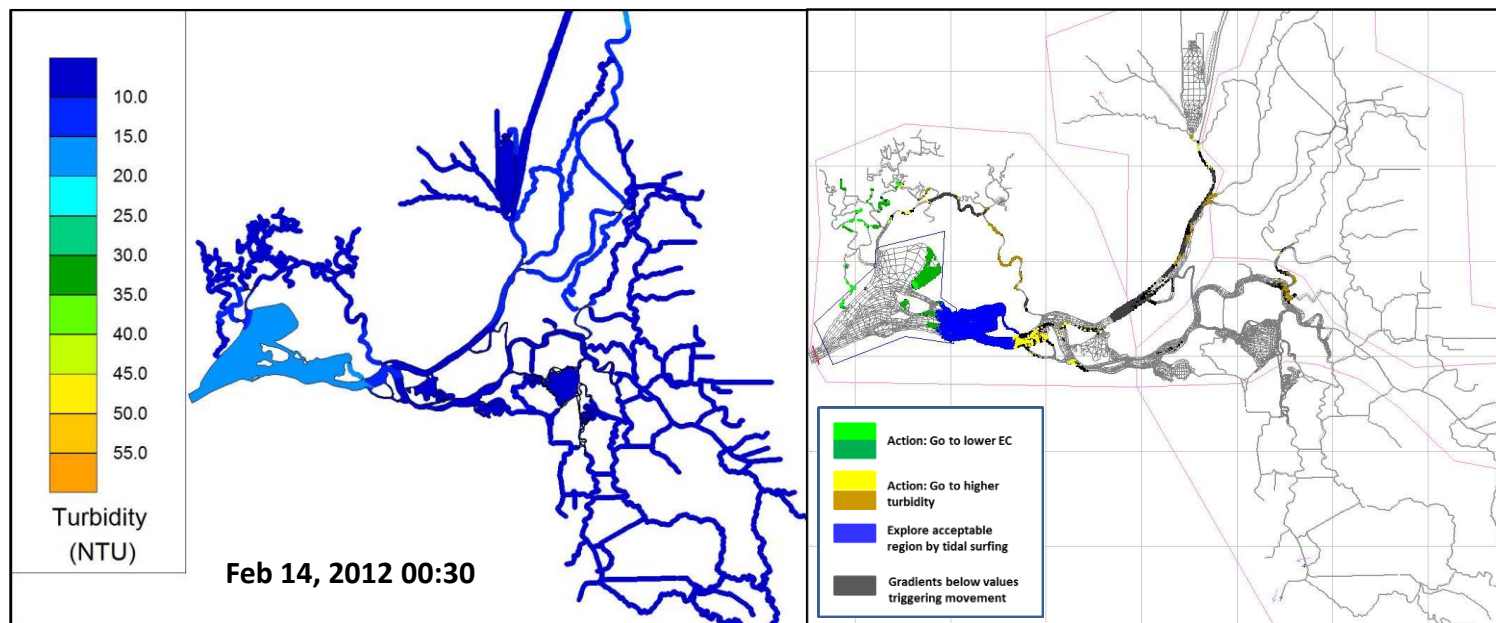
Figure 30 Turbidity contours and particle location in the RMA model grid on Feb. 14, 2012.
