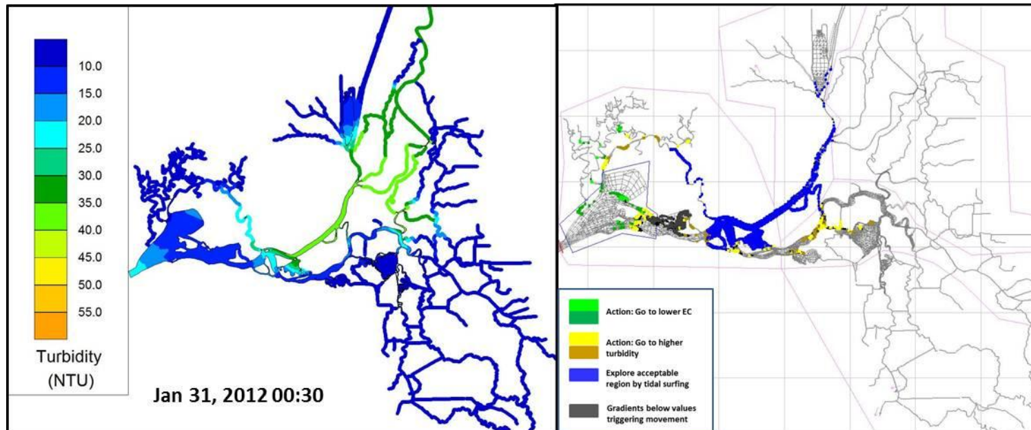
Figure 30 Turbidity contours and particle location in the RMA model grid on Jan. 31, 2012.
