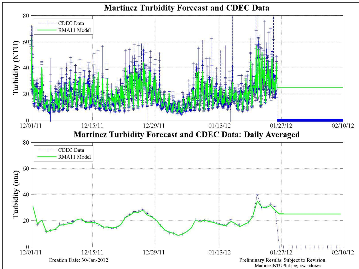
Figure 6 Martinez turbidity BC was compiled from CDEC data then extended linearly to a value of 25 NTU. Zero values indicate the end of data (blue).
