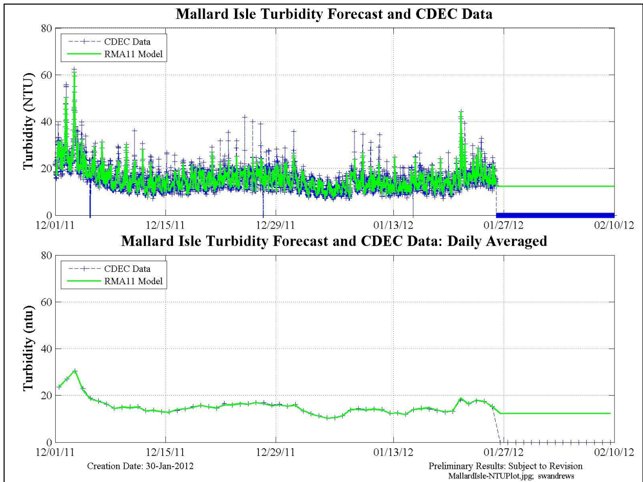
Figure 7 The Sacramento River at Mallard Island internal turbidity BC was compiled from CDEC data then extended linearly to a value of 12 NTU. Zero values indicate the end of data (blue).
