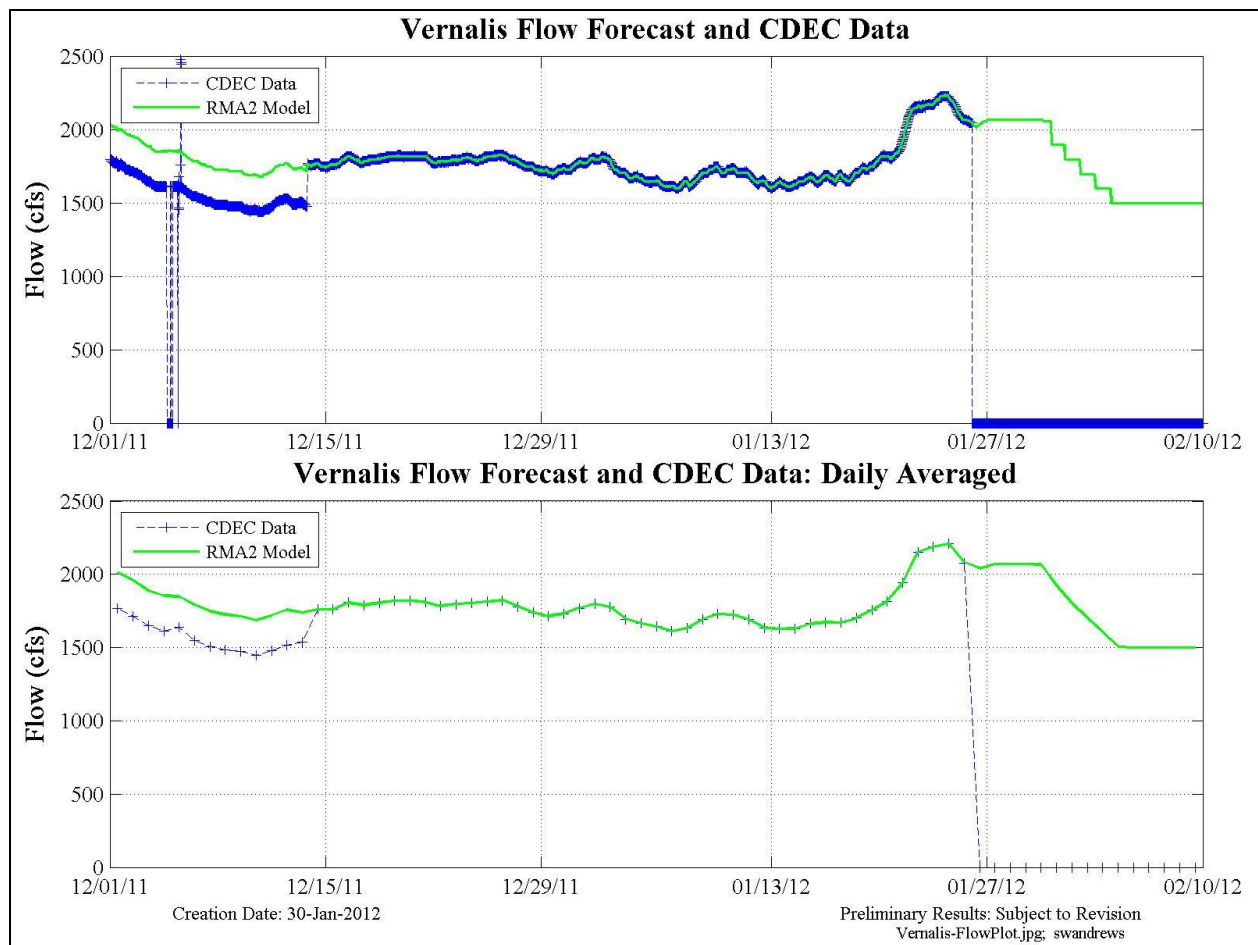
Figure 4 Vernalis flow BC was compiled using CDEC and USGS data and DWR DSM2 forecast flow. Zero values indicate the end of data (blue). The USGS rating for Vernalis changed Dec. 13, 2011 and is reflected in the RMA2 model flow. The flow was not shifted in the CDEC database prior to Dec. 13, 2011.
