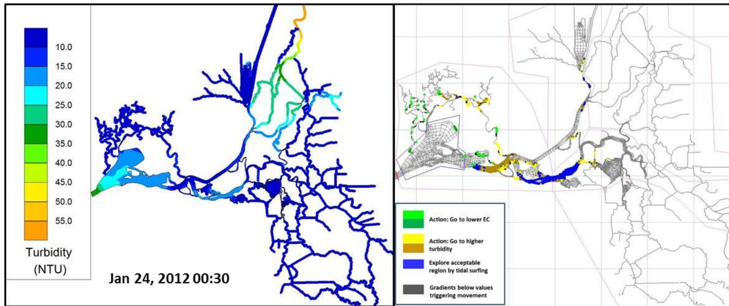
Figure 29 Turbidity contours and particle location in the RMA model grid on Jan. 24, 2012.
