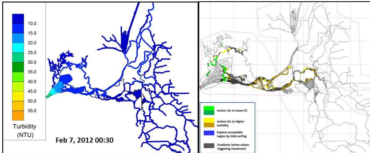
Figure 31 Turbidity contours and particle location in the RMA model grid on Feb. 7, 2012.
