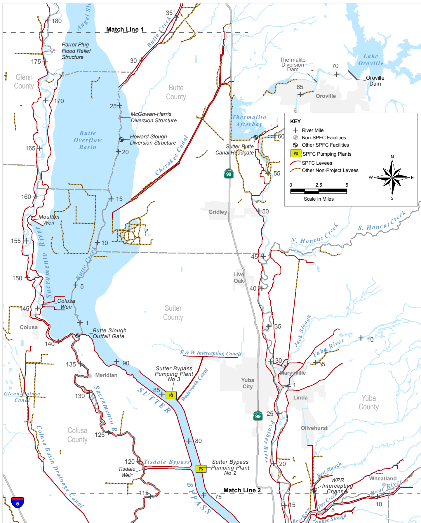
Detail 3. Sacramento River from the Parrott Plug Relief Structure to the Tisdale Bypass, Sutter Bypass, Butte Overflow Basin and the Feather River.
