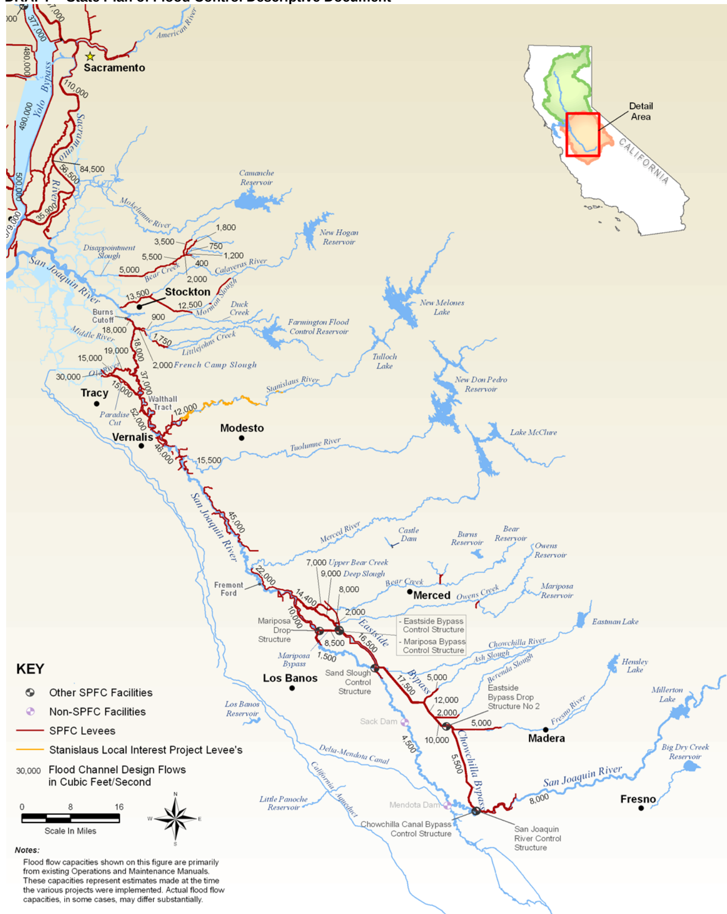
Figure 3-3. Design Flood Flow Capacities Within the San Joaquin River, Bypasses, and Major Tributaries and Distributaries in the San Joaquin River Basin
