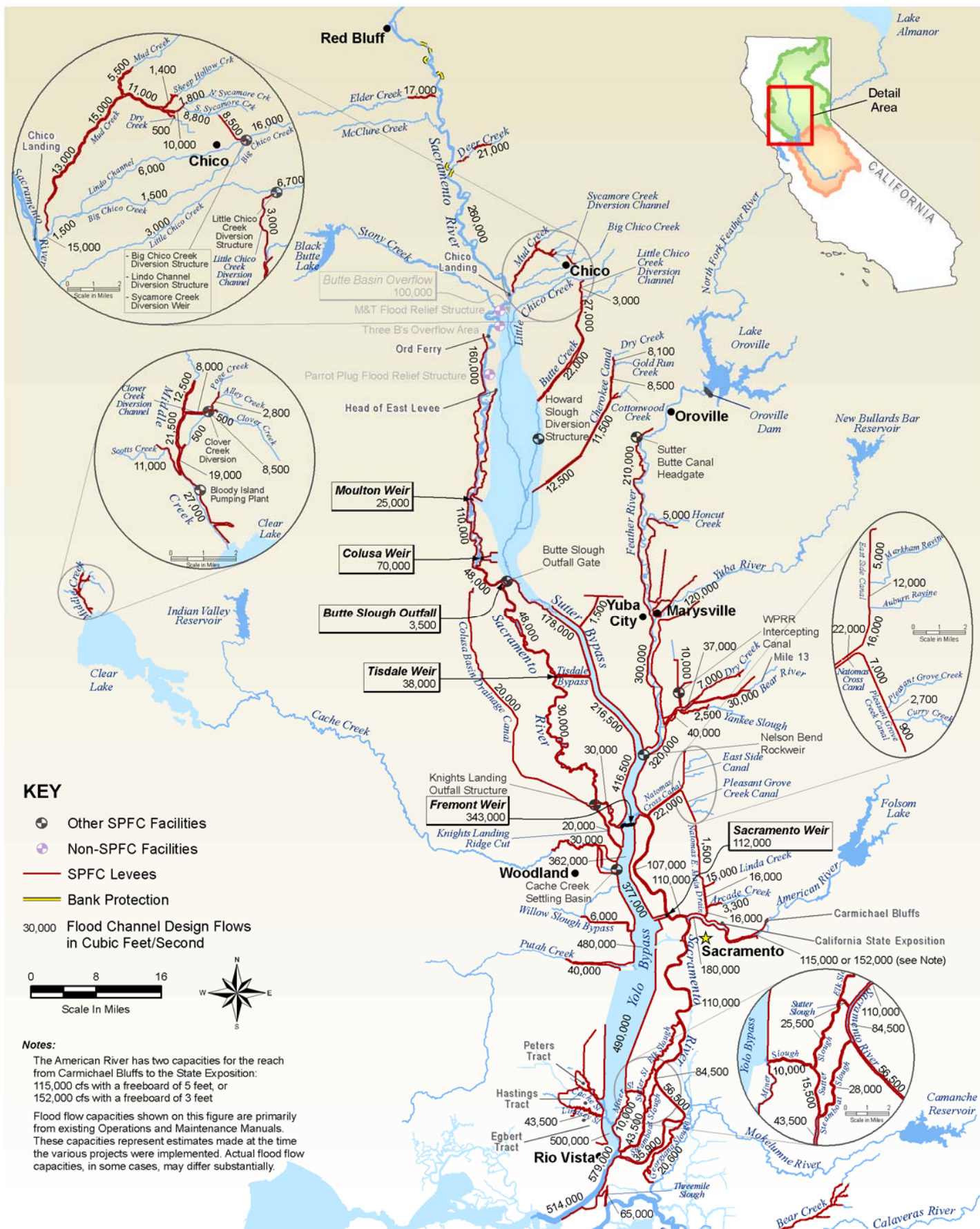
Figure 3-2. Design Flood Flow Capacities Within the Sacramento River, Bypasses, and Major Tributaries and Distributaries in the Sacramento River Basin January 2010
