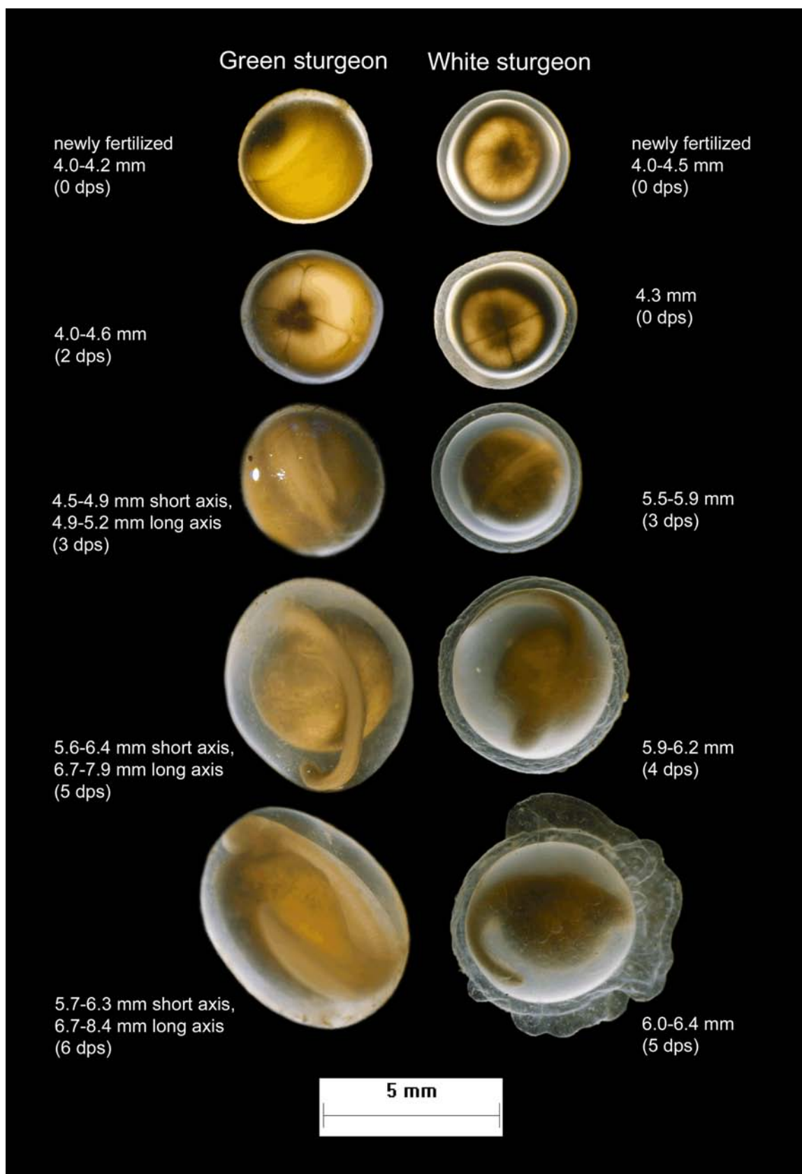
FIGURE 3 — Comparing the eggs of green (left) and white (right) sturgeons. Green sturgeon eggs were provided by Joel Van Eenennaam, UCD, and incubated at 15.5 °C. White sturgeon eggs were provided by Stoltz Sea Farm, Galt, California, and incubated at 16 °C. Eggs developed and were photographed at the TFCF at 18 – 19 °C. dps = days post spawn. Reclamation photographs by René C. Reyes.
